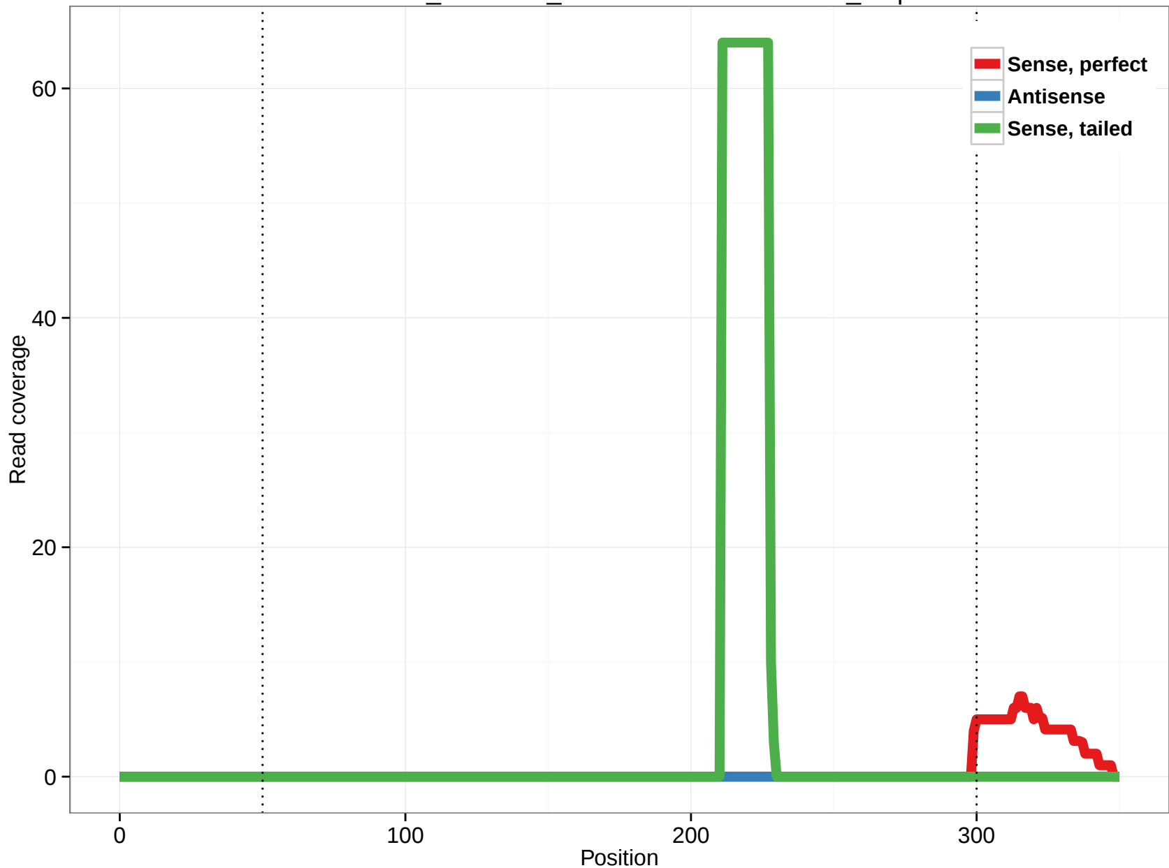
ornAna1_ensGene_ENSOANT00000013548_1.3p
