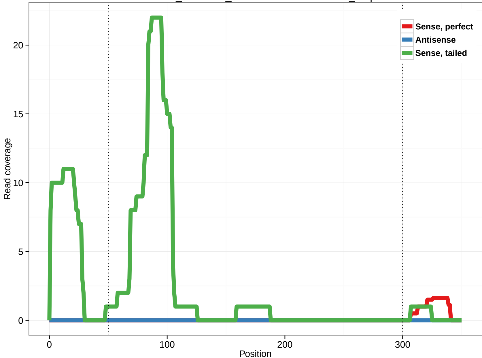
ornAna1_ensGene_ENSOANT00000013417_3.3p
