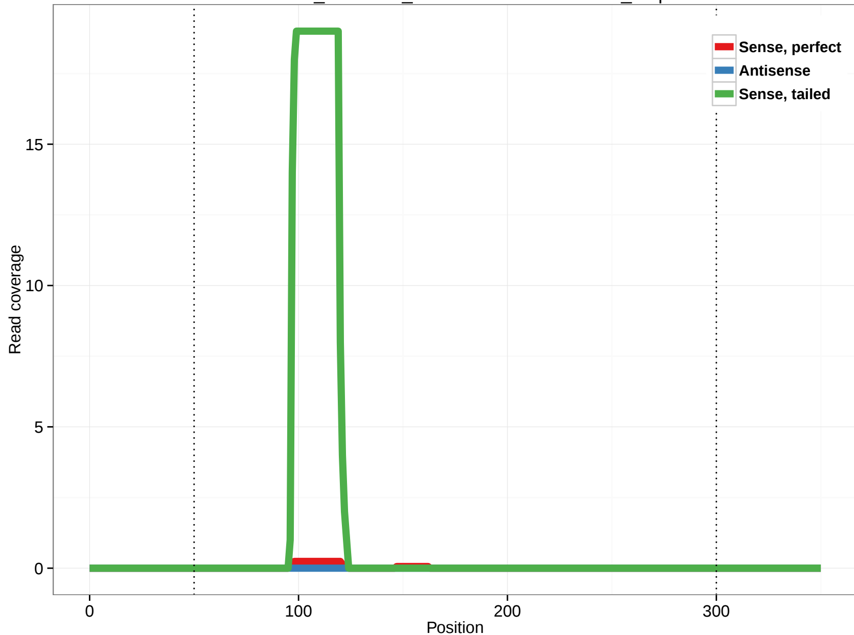
ornAna1_ensGene_ENSOANT00000013417_2.3p
