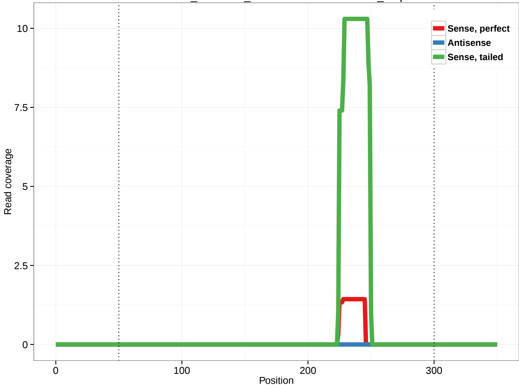
ornAna1_ensGene_ENSOANT00000013311_3.5p
