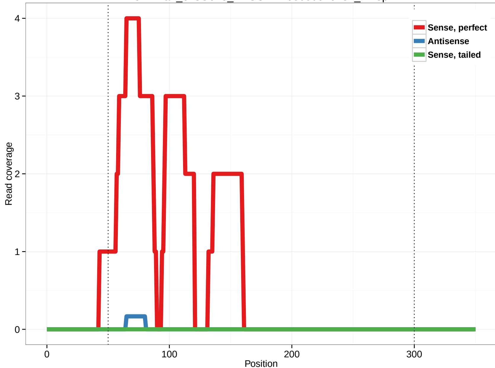
ornAna1_ensGene_ENSOANT00000013282_11.3p
