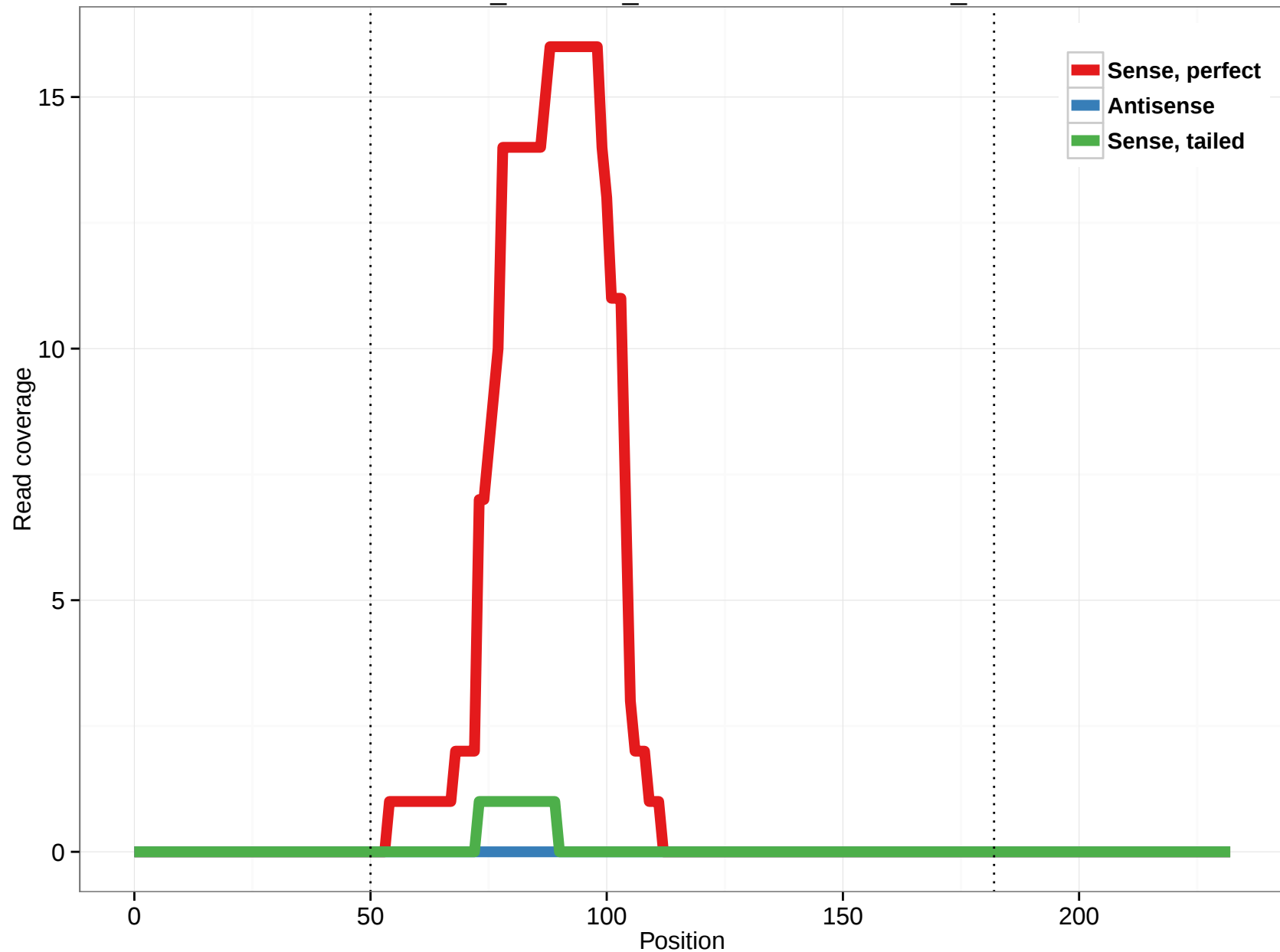
ornAna1_ensGene_ENSOANT00000013134_4
