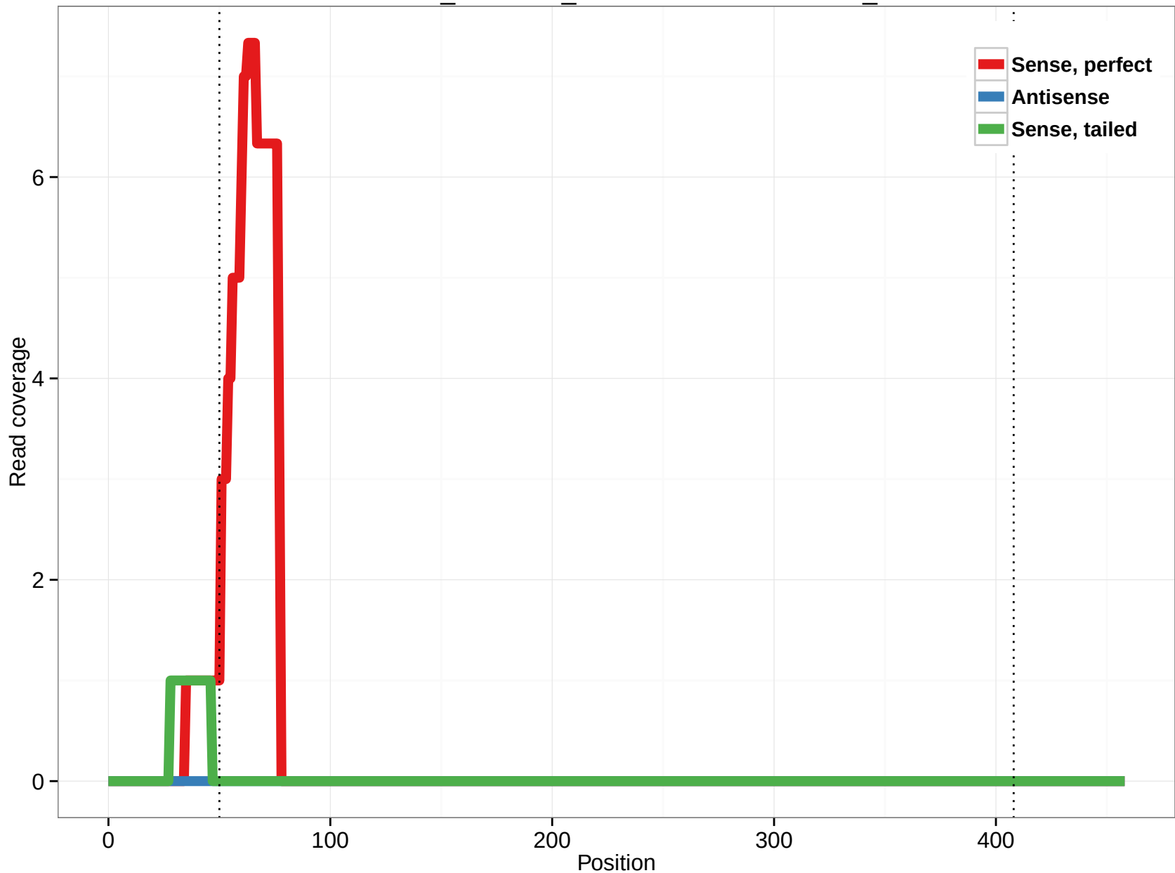
ornAna1_ensGene_ENSOANT00000013134_1
