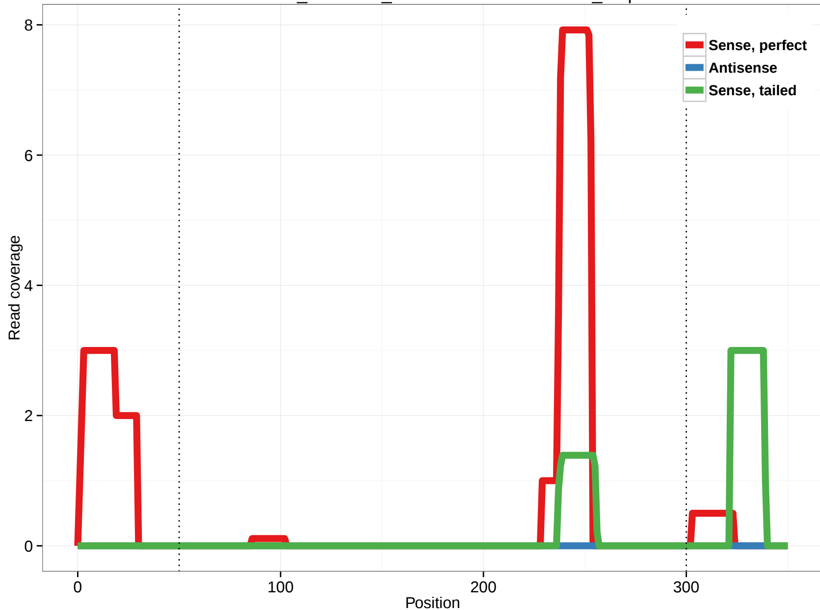
ornAna1_ensGene_ENSOANT00000013125_9.3p
