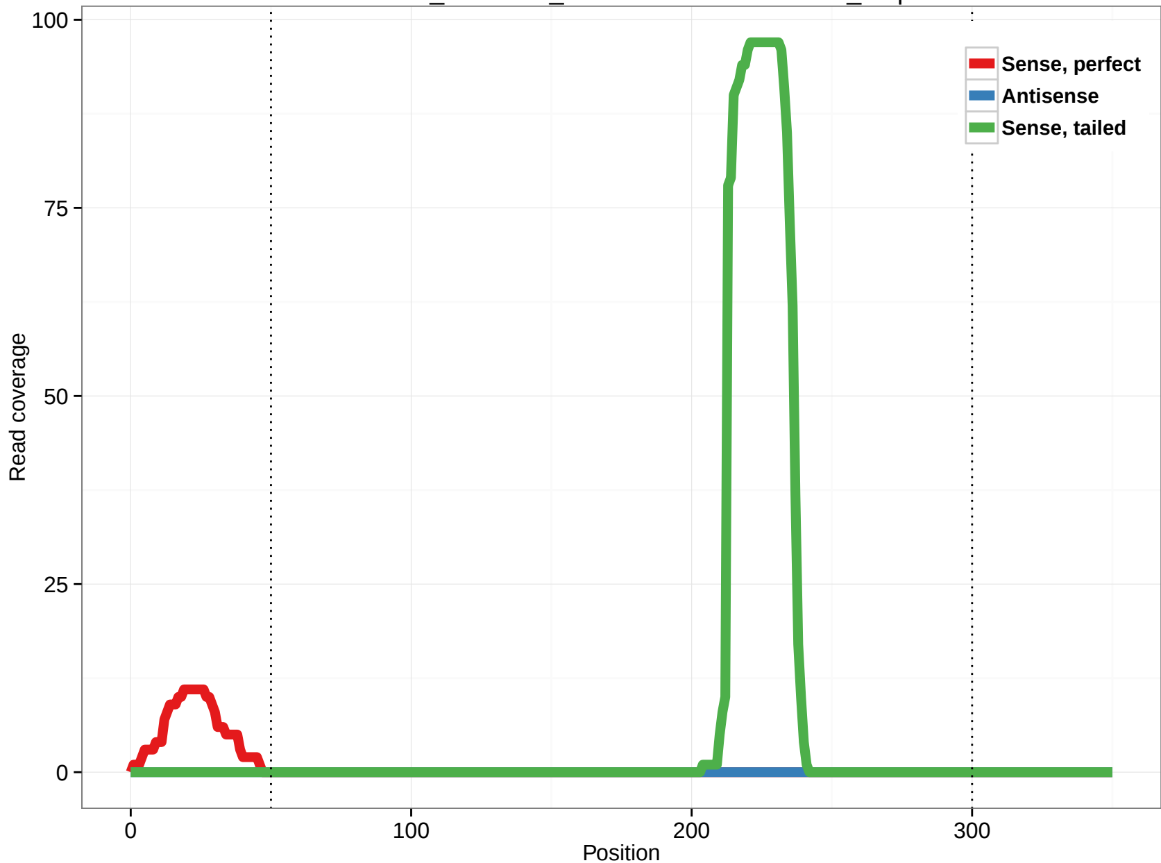
ornAna1_ensGene_ENSOANT00000013125_6.5p
