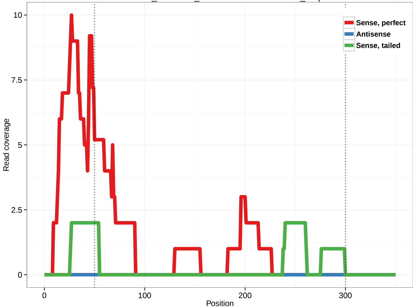
ornAna1_ensGene_ENSOANT00000013125_3.5p
