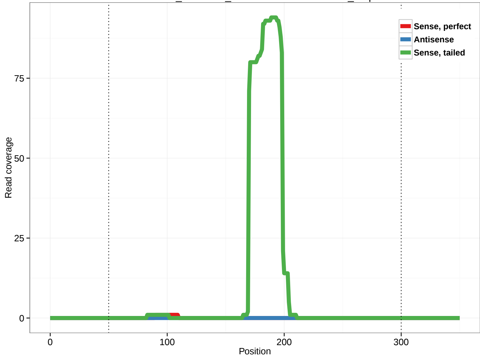
ornAna1_ensGene_ENSOANT00000013089_2.3p
