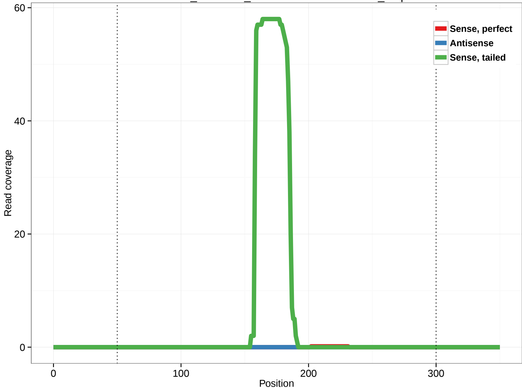
ornAna1_ensGene_ENSOANT00000013060_6.5p
