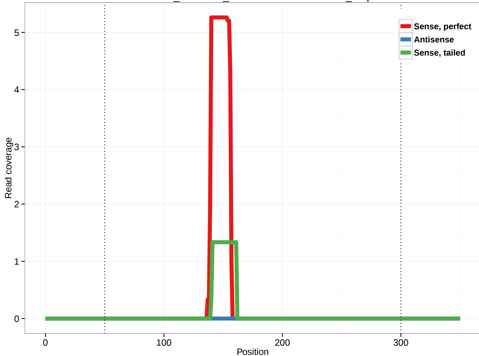
ornAna1_ensGene_ENSOANT00000013058_2.3p
