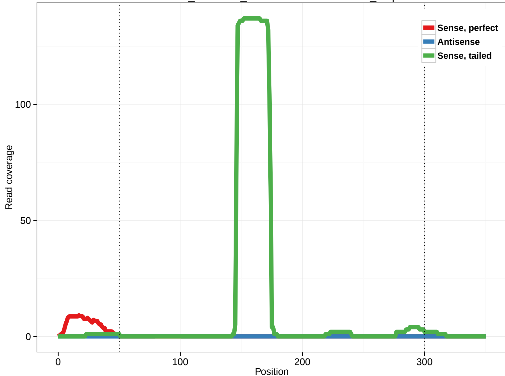
ornAna1_ensGene_ENSOANT00000013038_3.5p
