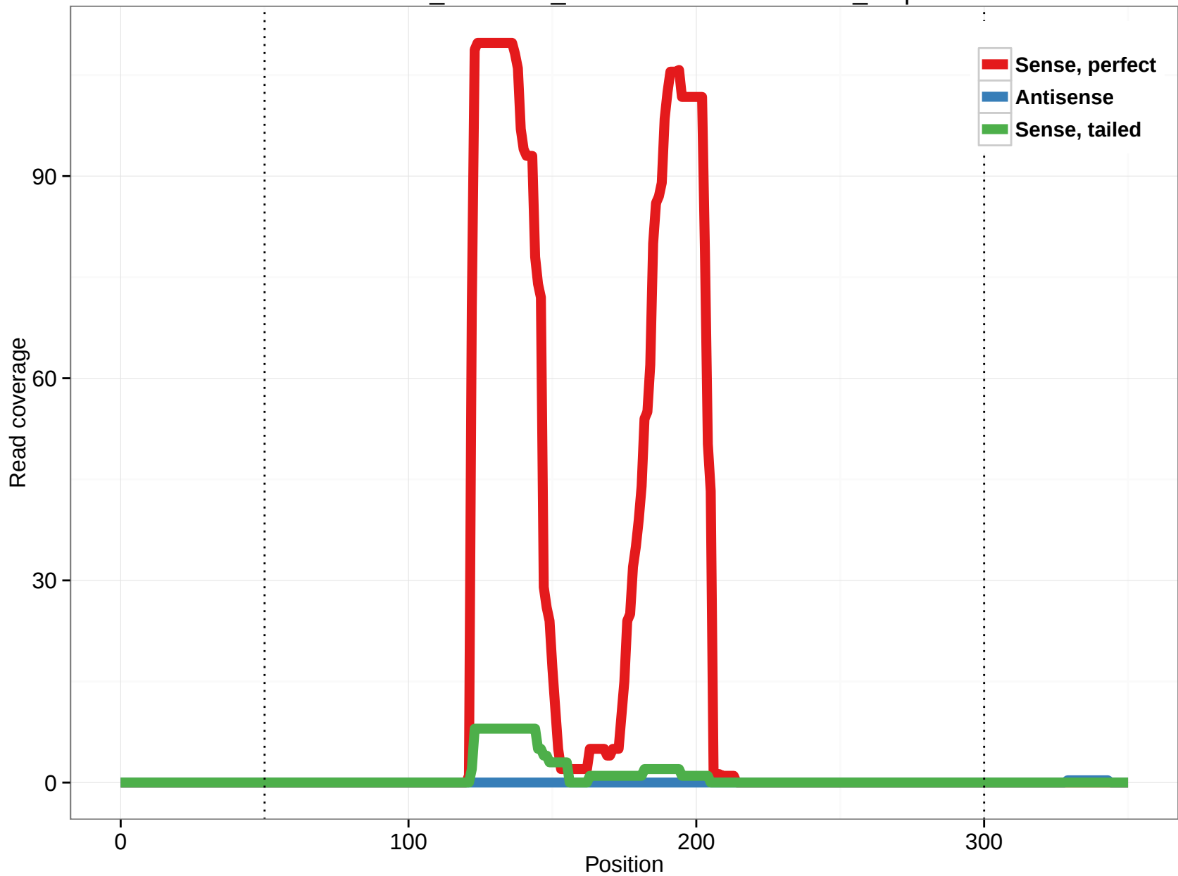
ornAna1_ensGene_ENSOANT00000013022_4.3p
