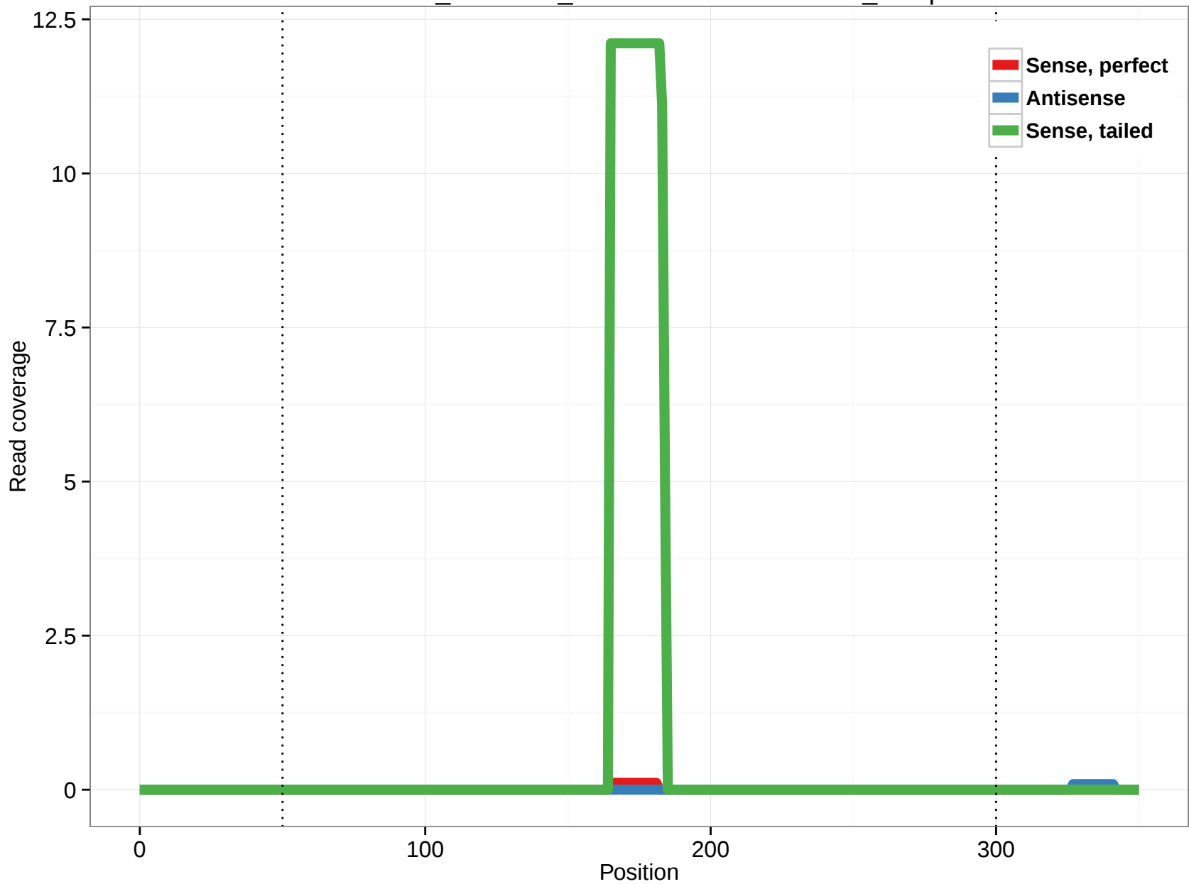
ornAna1_ensGene_ENSOANT00000013020_21.5p
