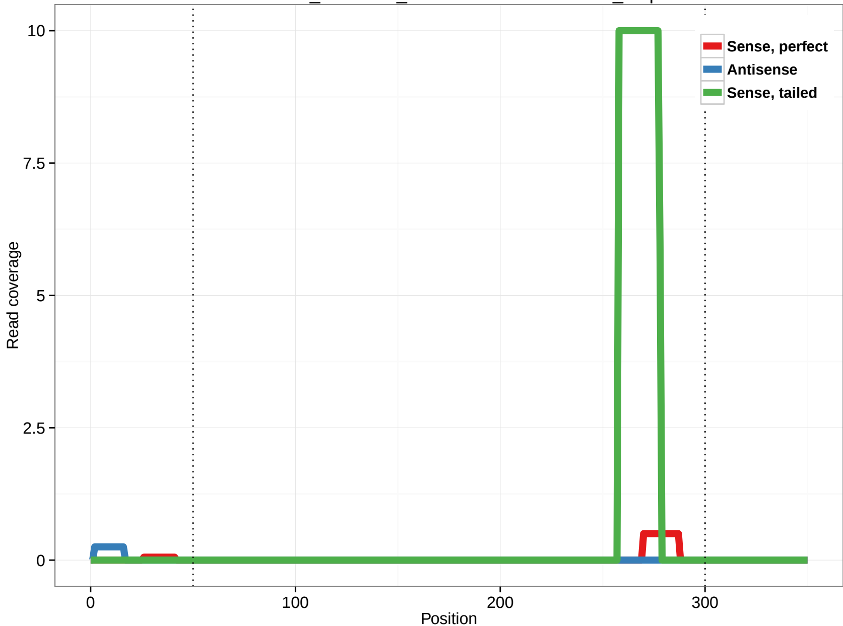
ornAna1_ensGene_ENSOANT00000012999_0.5p
