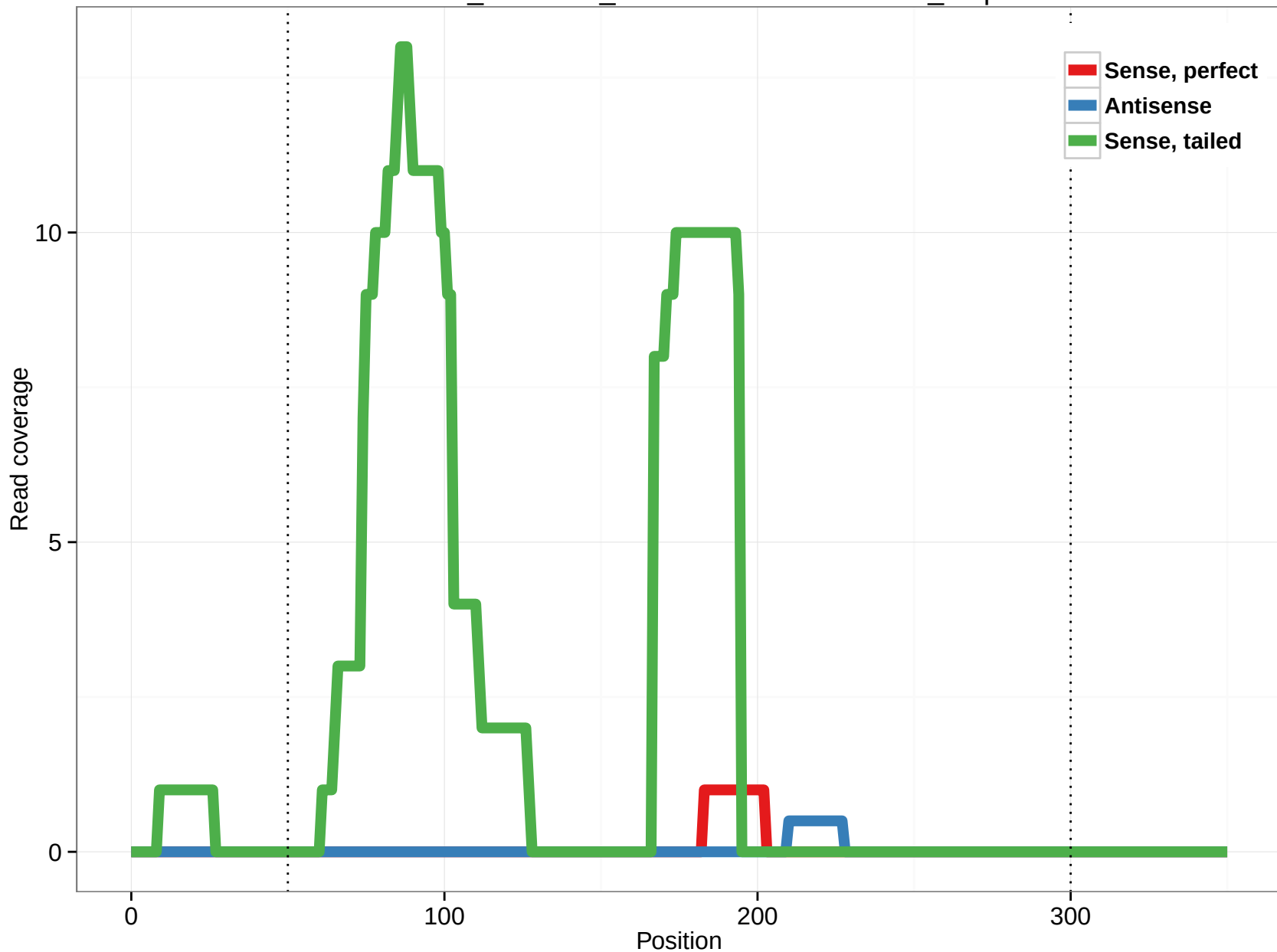
ornAna1_ensGene_ENSOANT00000012995_6.3p
