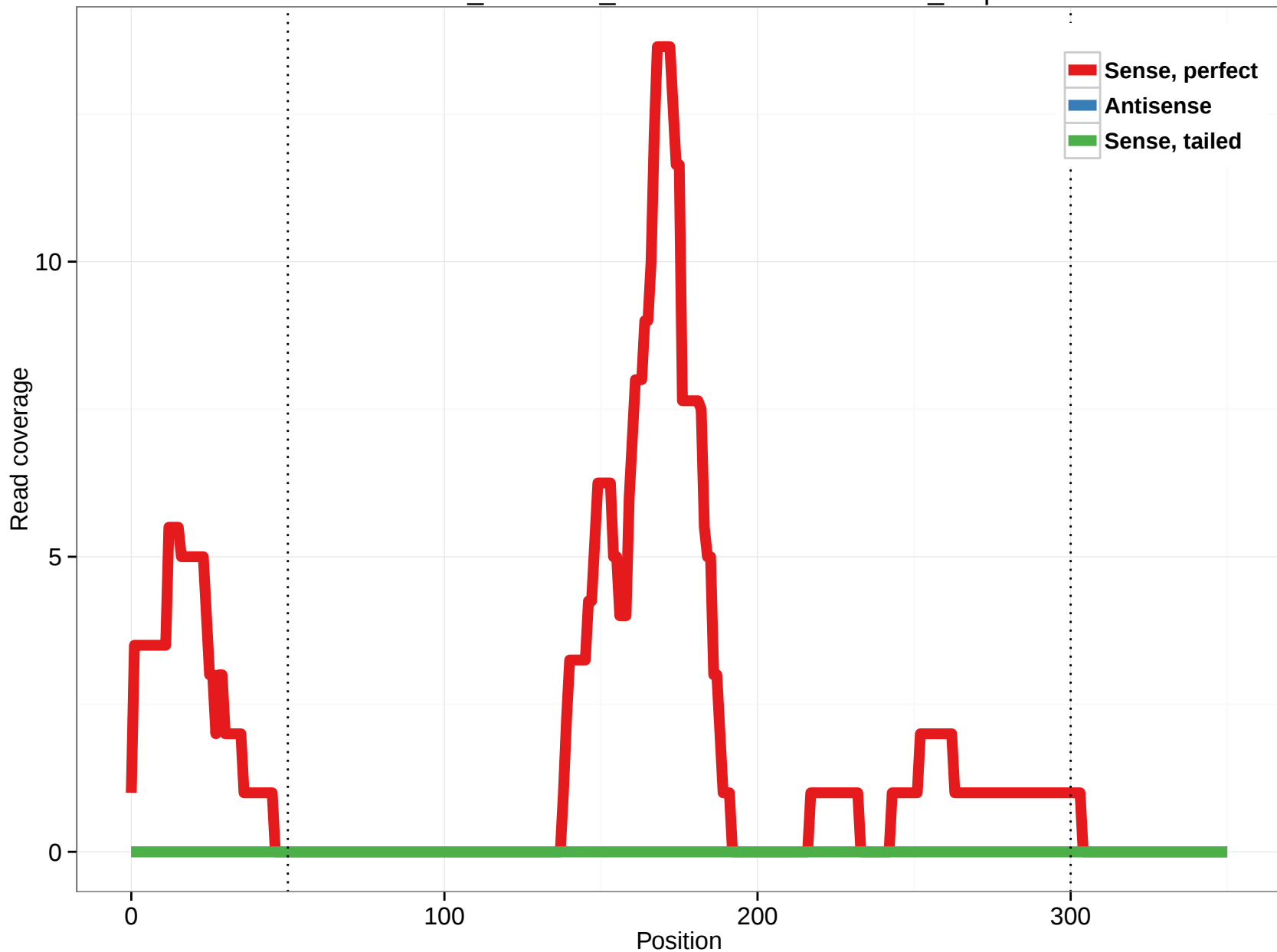
ornAna1_ensGene_ENSOANT00000012965_1.5p
