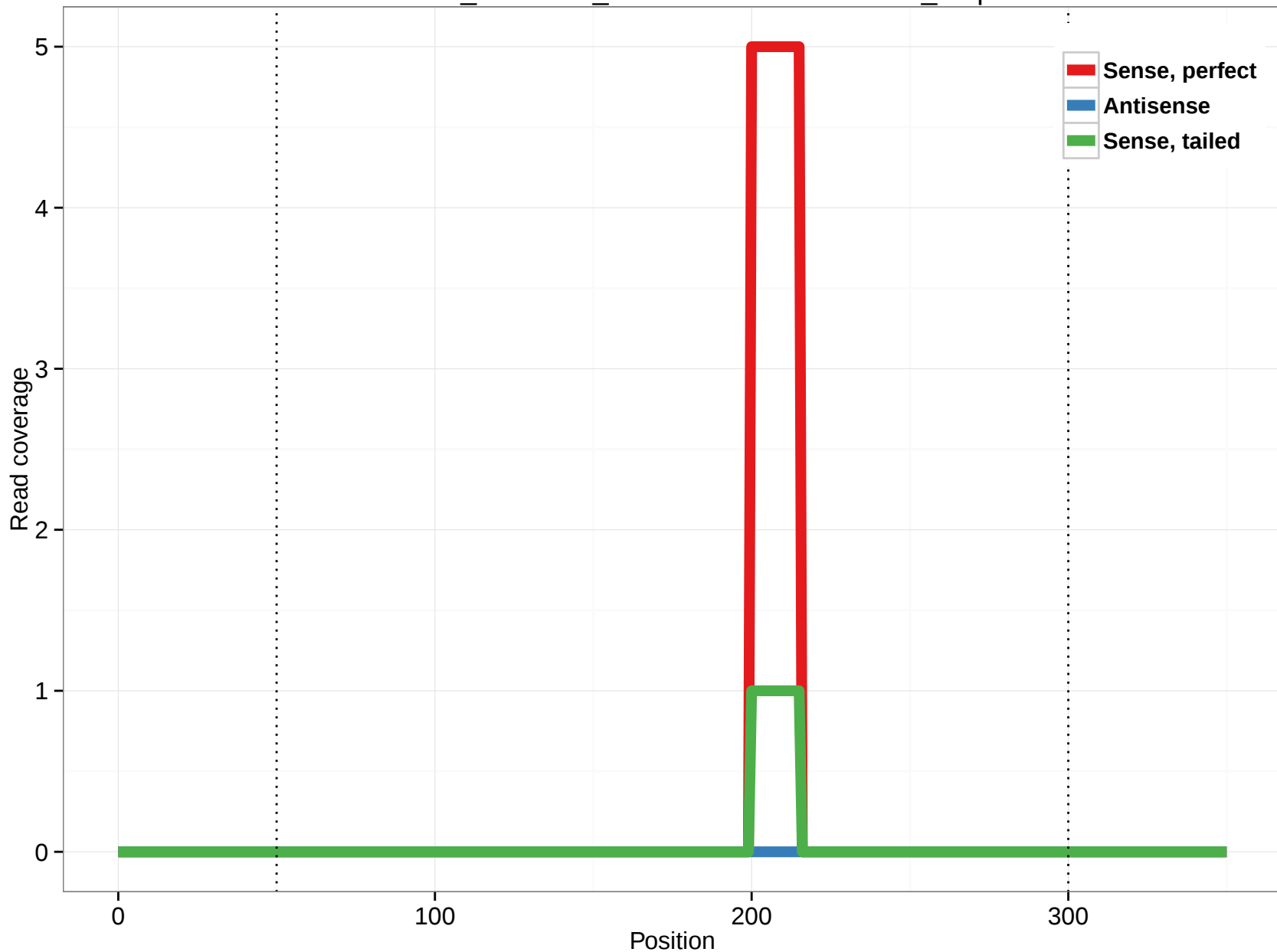
ornAna1_ensGene_ENSOANT00000012958_7.5p
