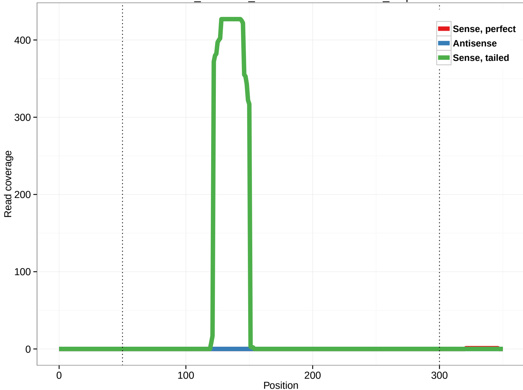
ornAna1_ensGene_ENSOANT00000012917_9.3p
