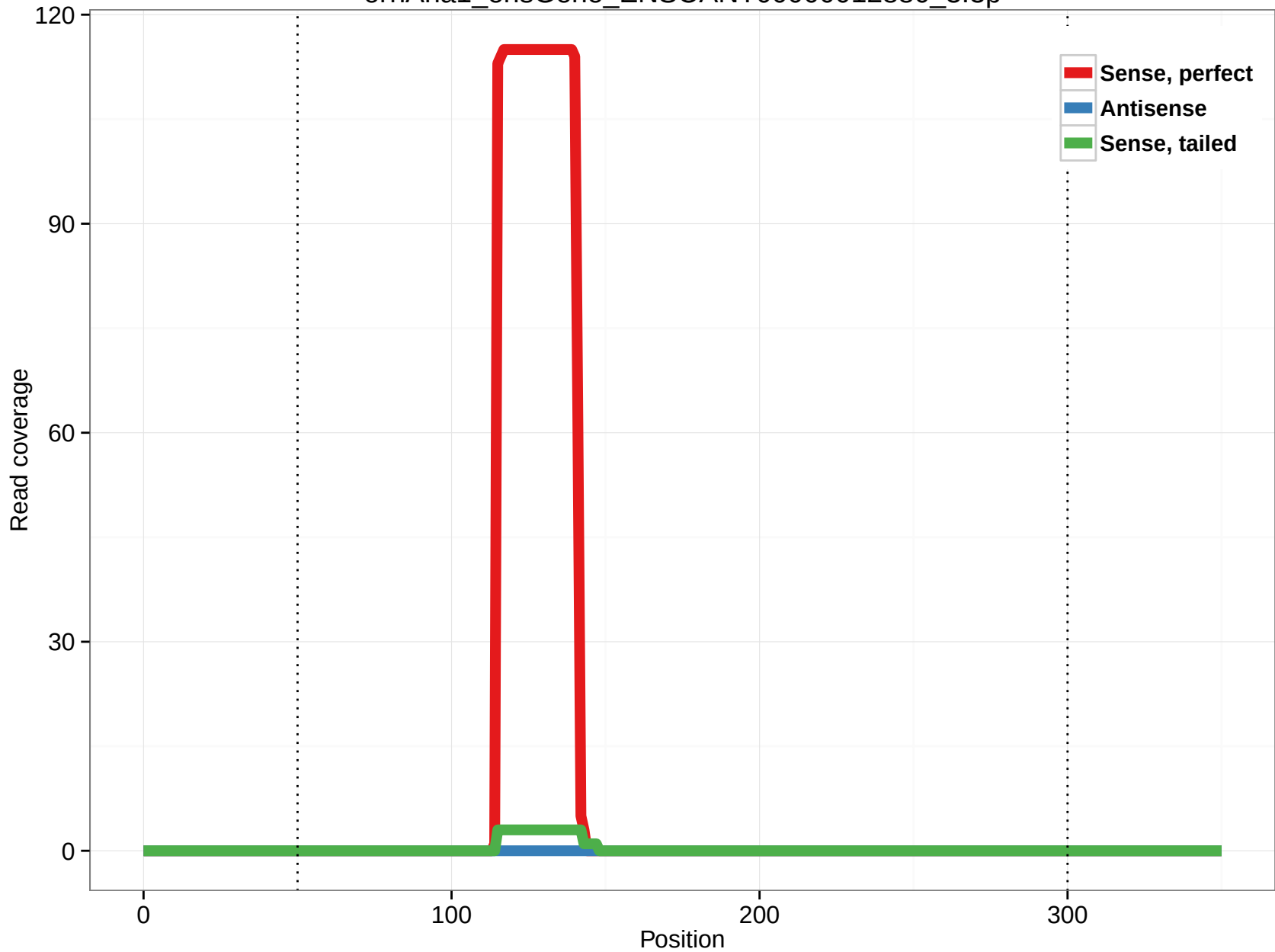
ornAna1_ensGene_ENSOANT00000012880_3.3p
