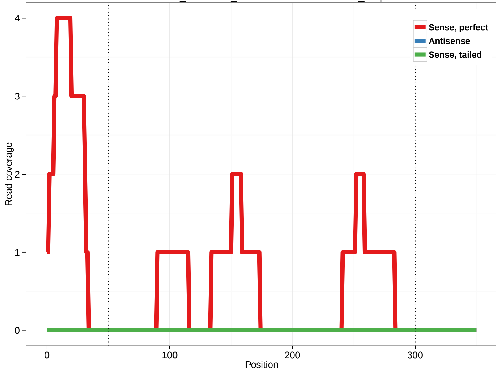
ornAna1_ensGene_ENSOANT00000012876_5.5p
