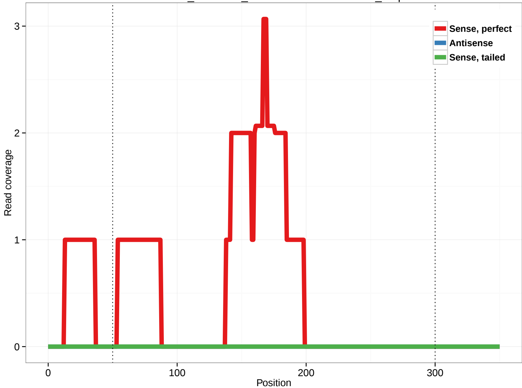
ornAna1_ensGene_ENSOANT00000012876_3.3p
