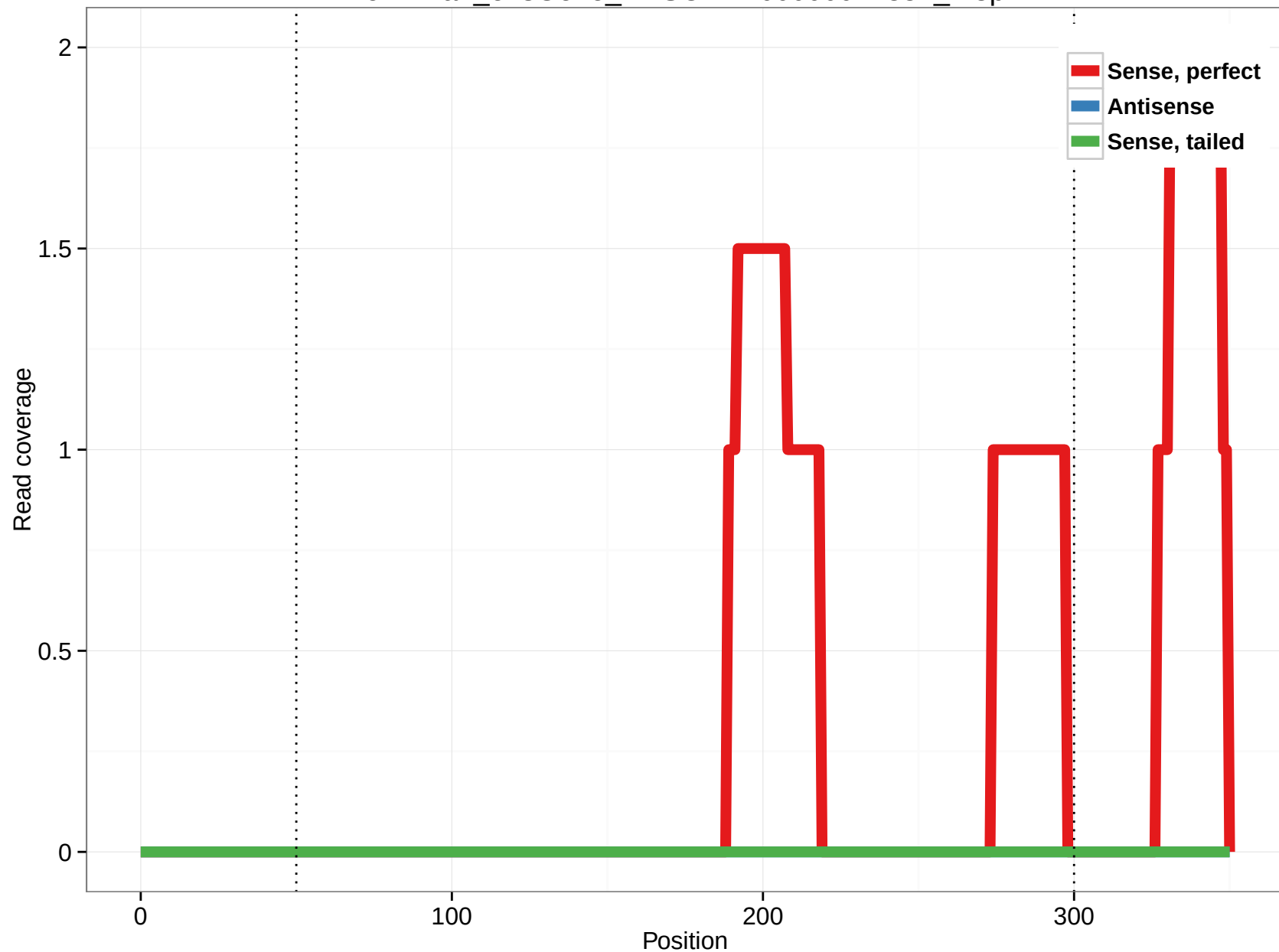
ornAna1_ensGene_ENSOANT00000012831_2.3p
