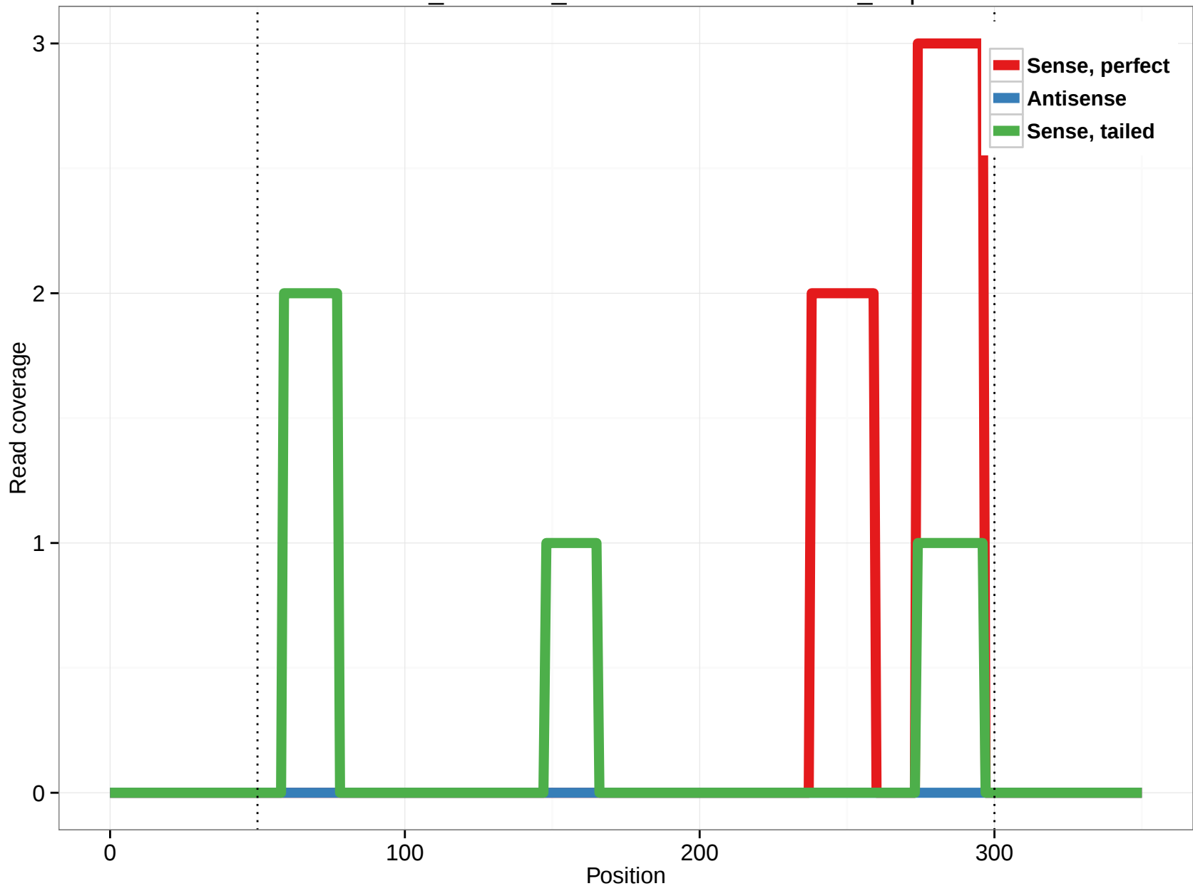
ornAna1_ensGene_ENSOANT00000012795_5.3p
