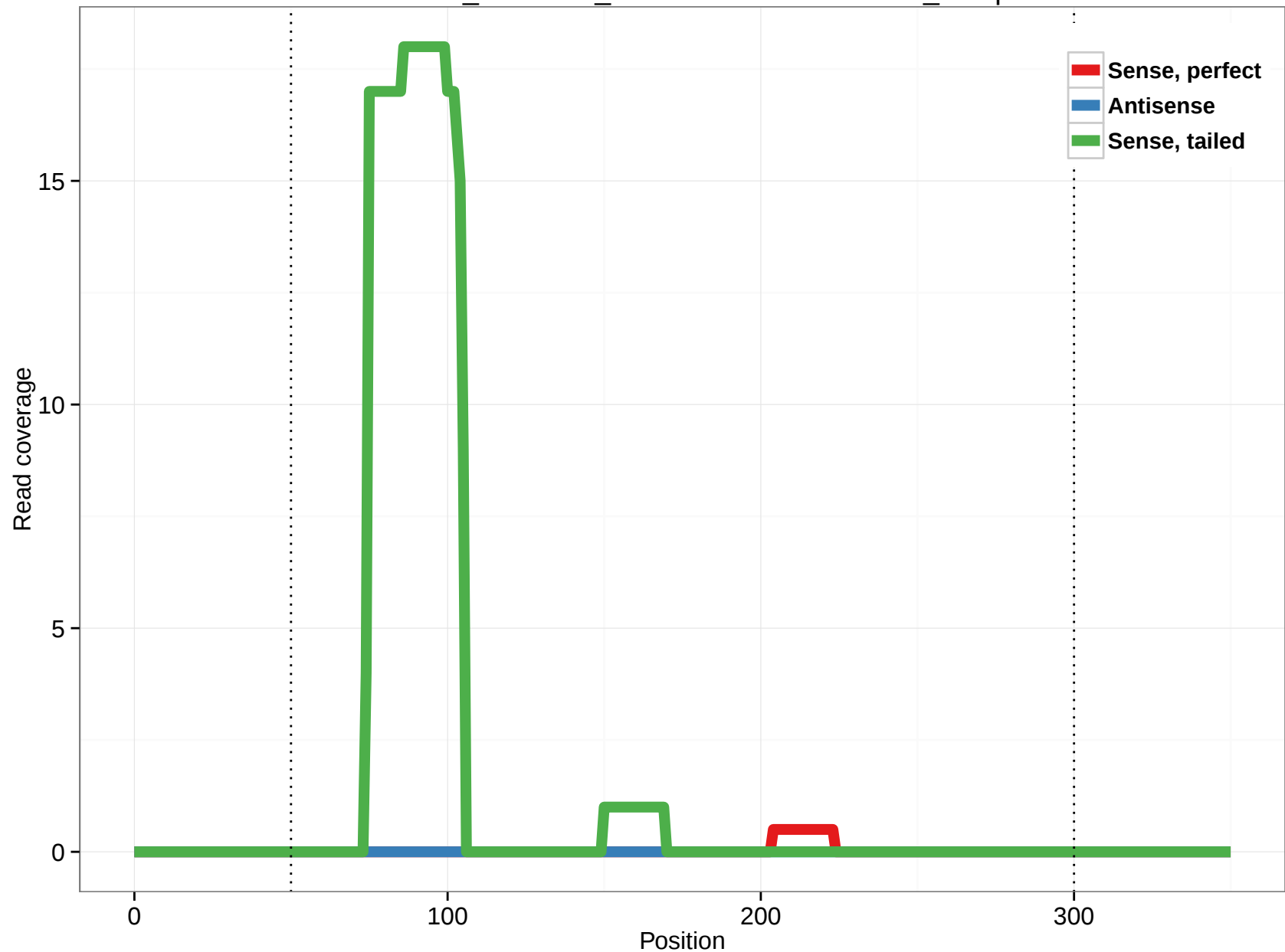
ornAna1_ensGene_ENSOANT00000012773_10.3p
