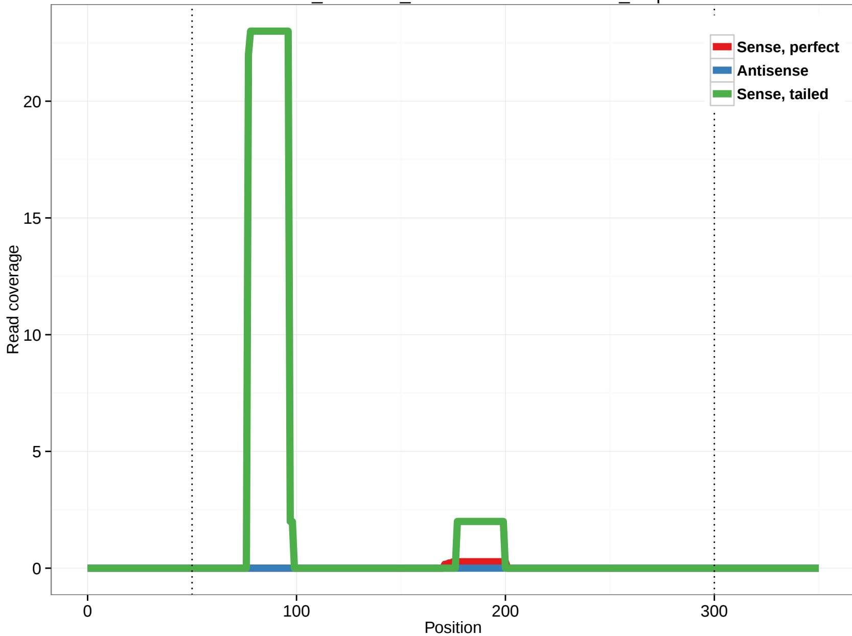
ornAna1_ensGene_ENSOANT00000012763_2.3p
