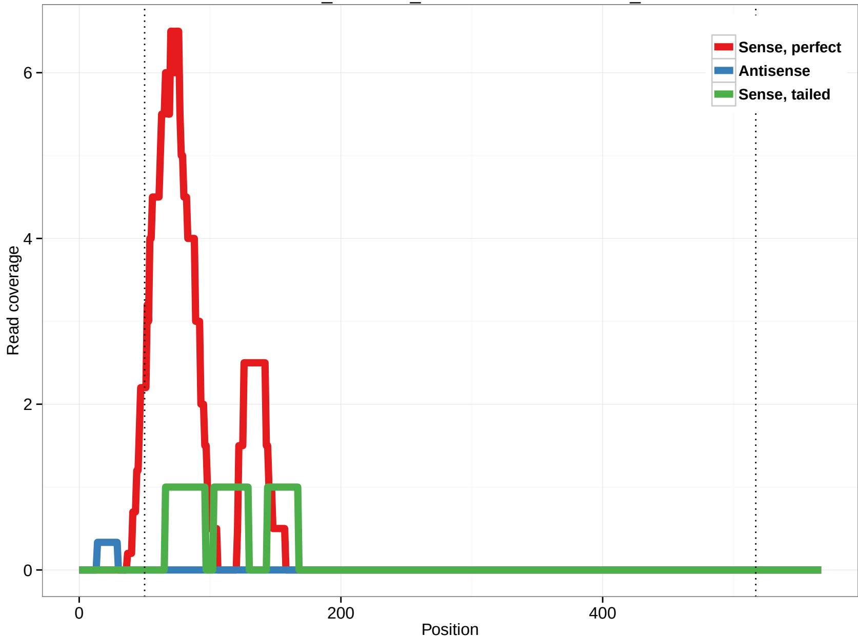
ornAna1_ensGene_ENSOANT00000012714_2
