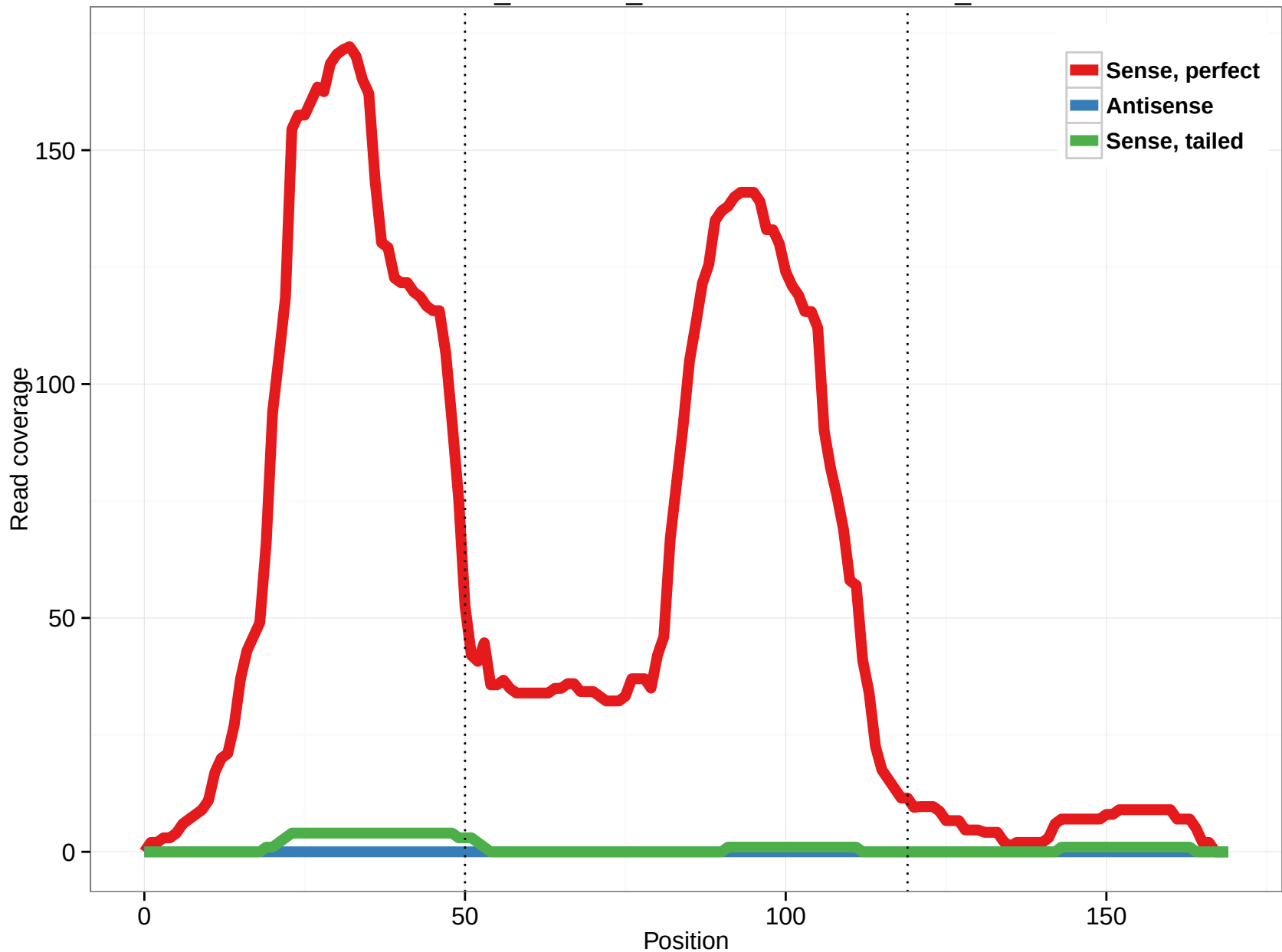
ornAna1_ensGene_ENSOANT00000012556_8
