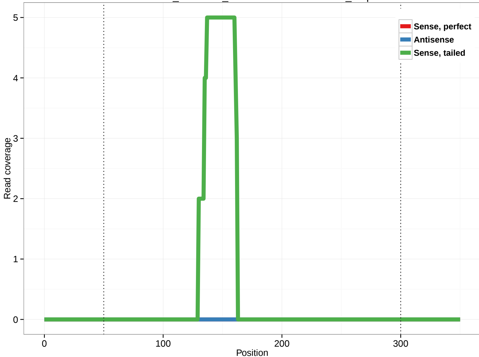
ornAna1_ensGene_ENSOANT00000012532_7.3p
