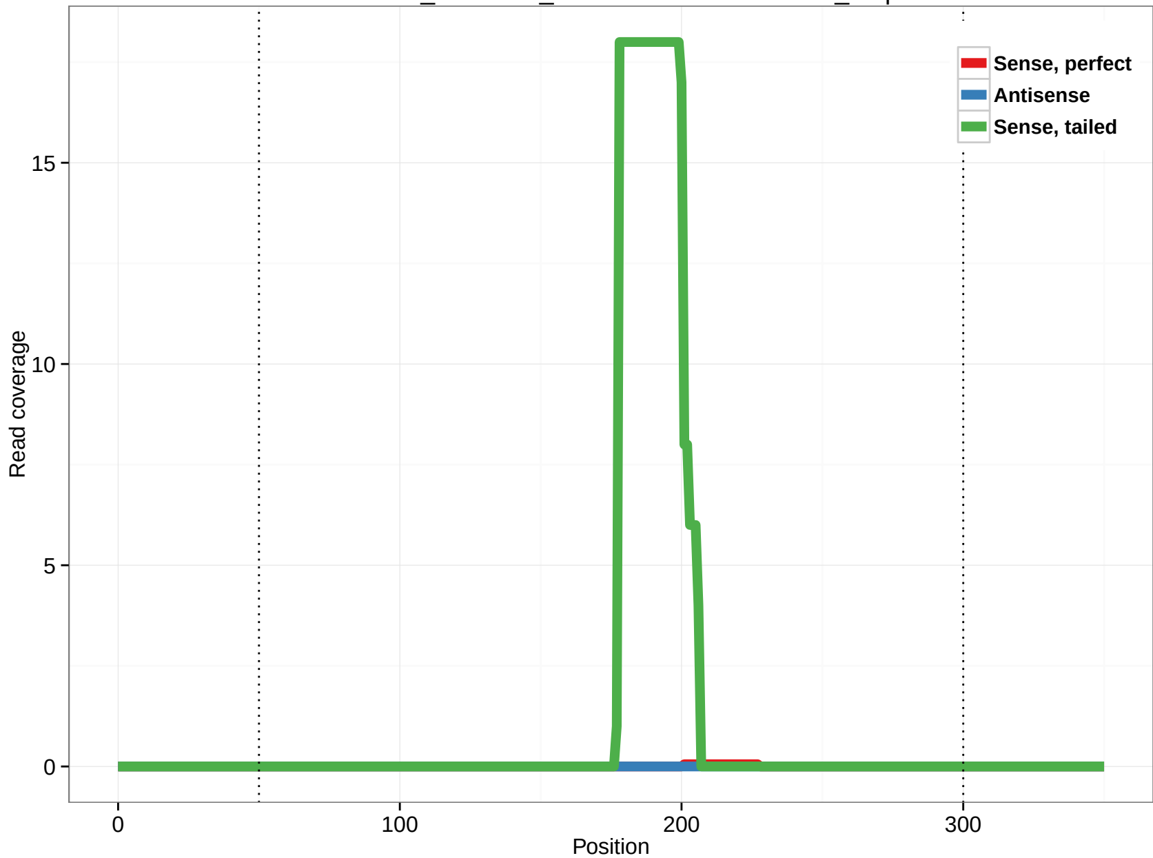
ornAna1_ensGene_ENSOANT00000012465_0.3p
