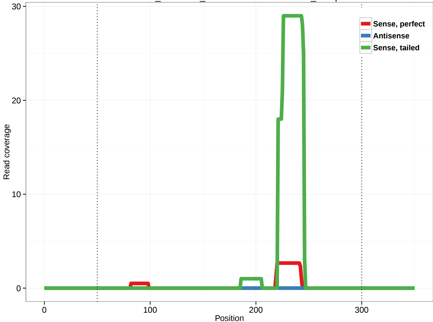
ornAna1_ensGene_ENSOANT00000012450_15.5p
