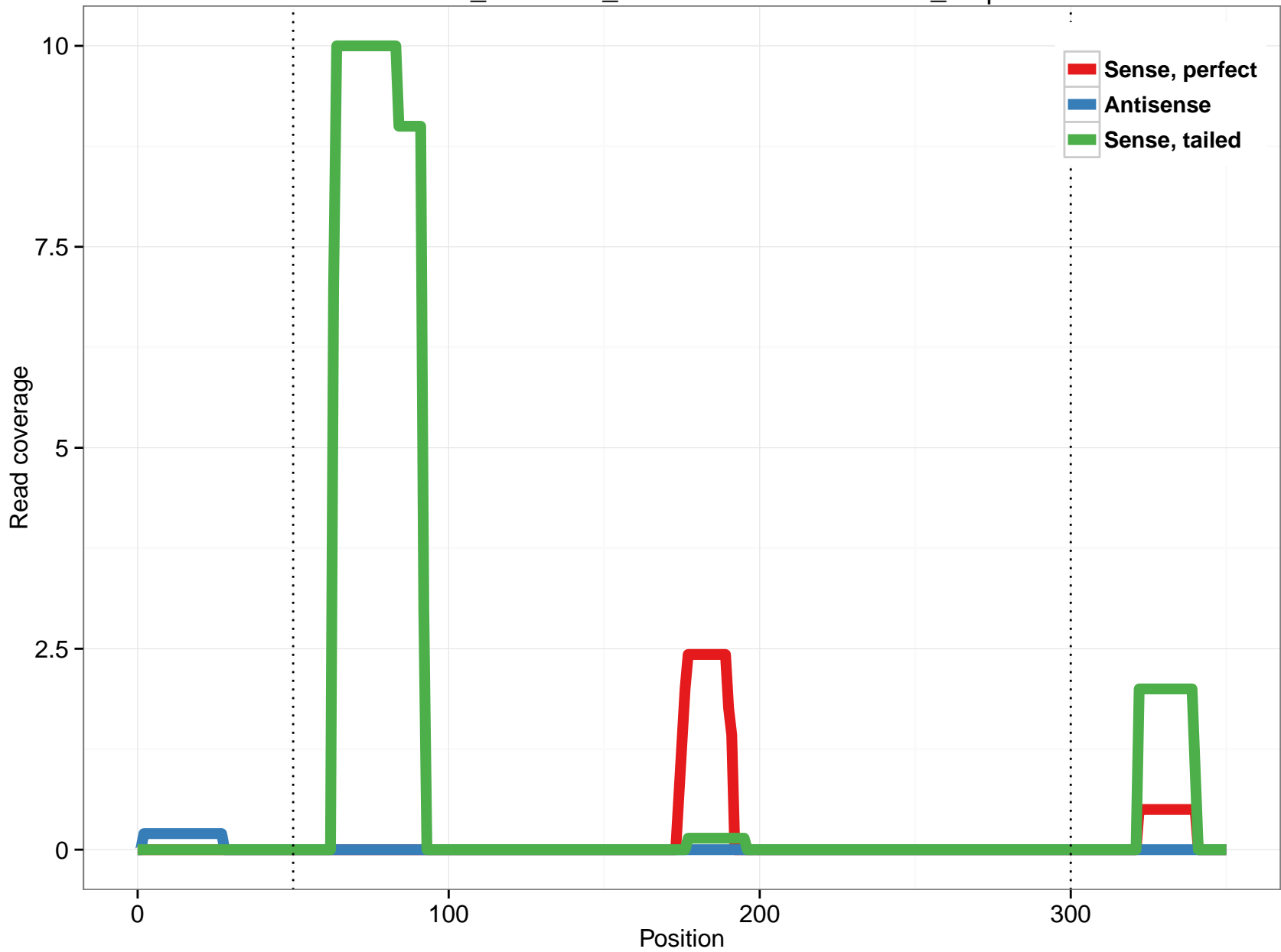
ornAna1_ensGene_ENSOANT00000012408_4.3p
