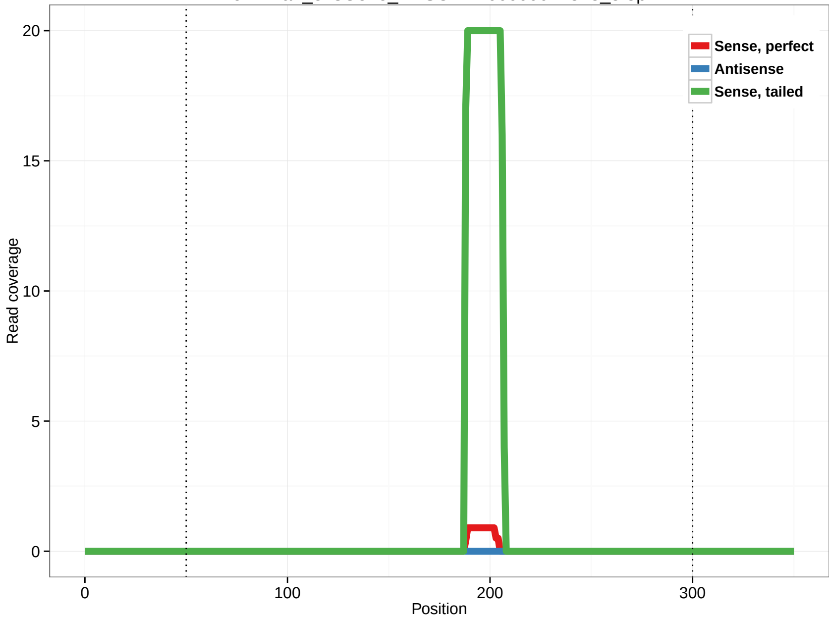
ornAna1_ensGene_ENSOANT00000012375_5.5p
