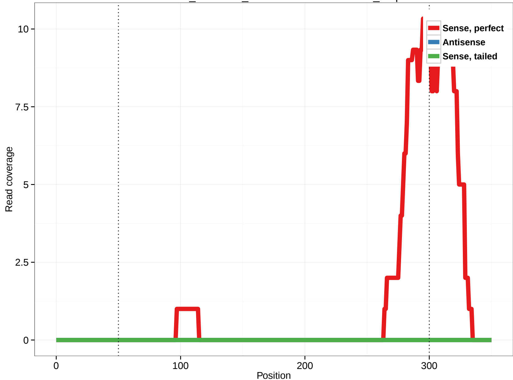
ornAna1_ensGene_ENSOANT00000012334_1.3p
