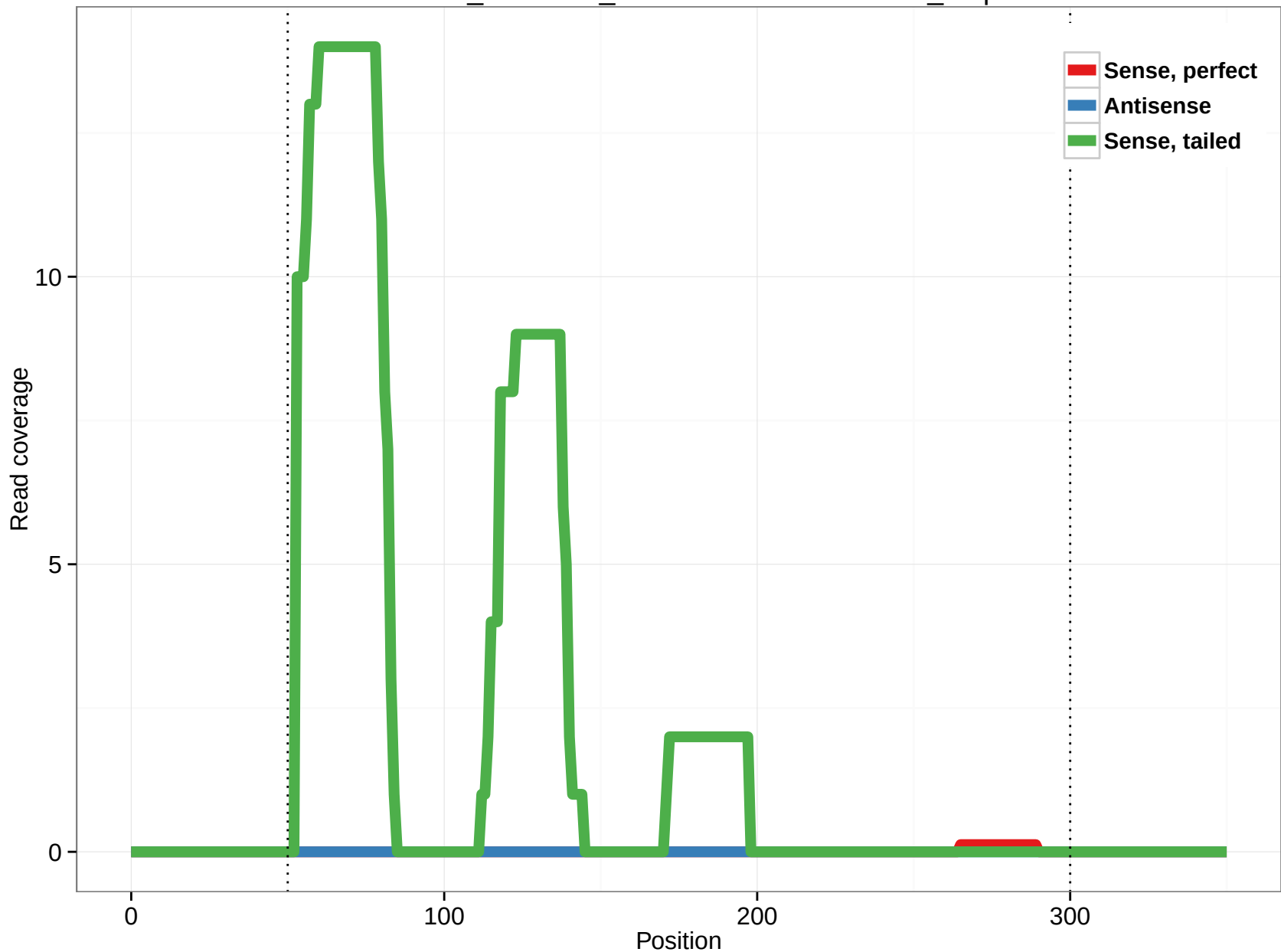
ornAna1_ensGene_ENSOANT00000012308_4.3p
