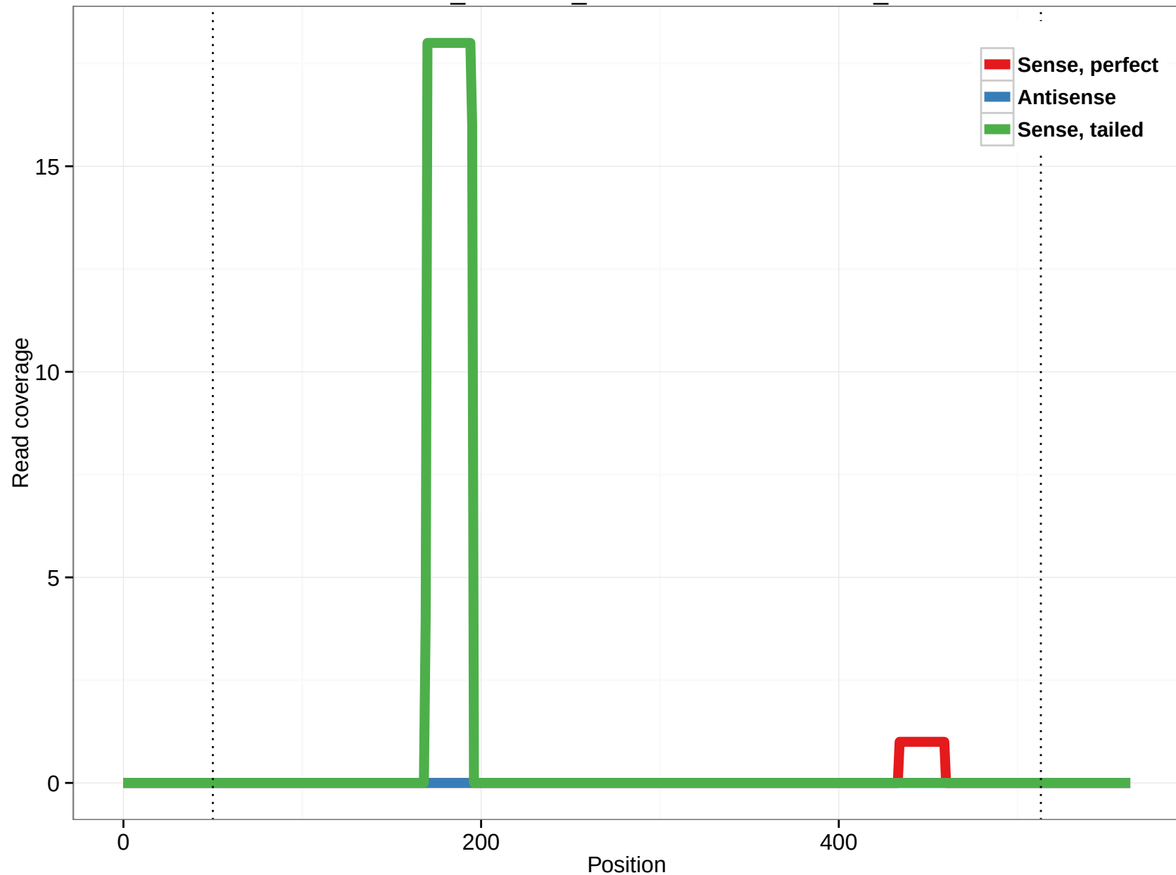
ornAna1_ensGene_ENSOANT00000012288_1
