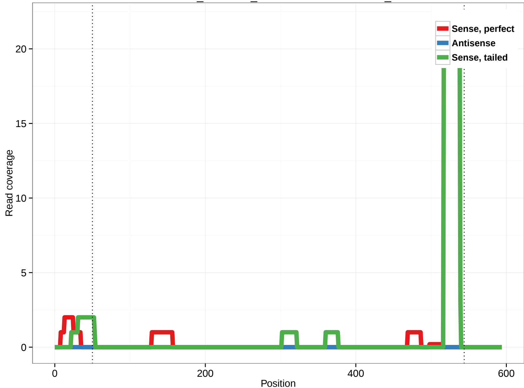
ornAna1_ensGene_ENSOANT00000012286_17
