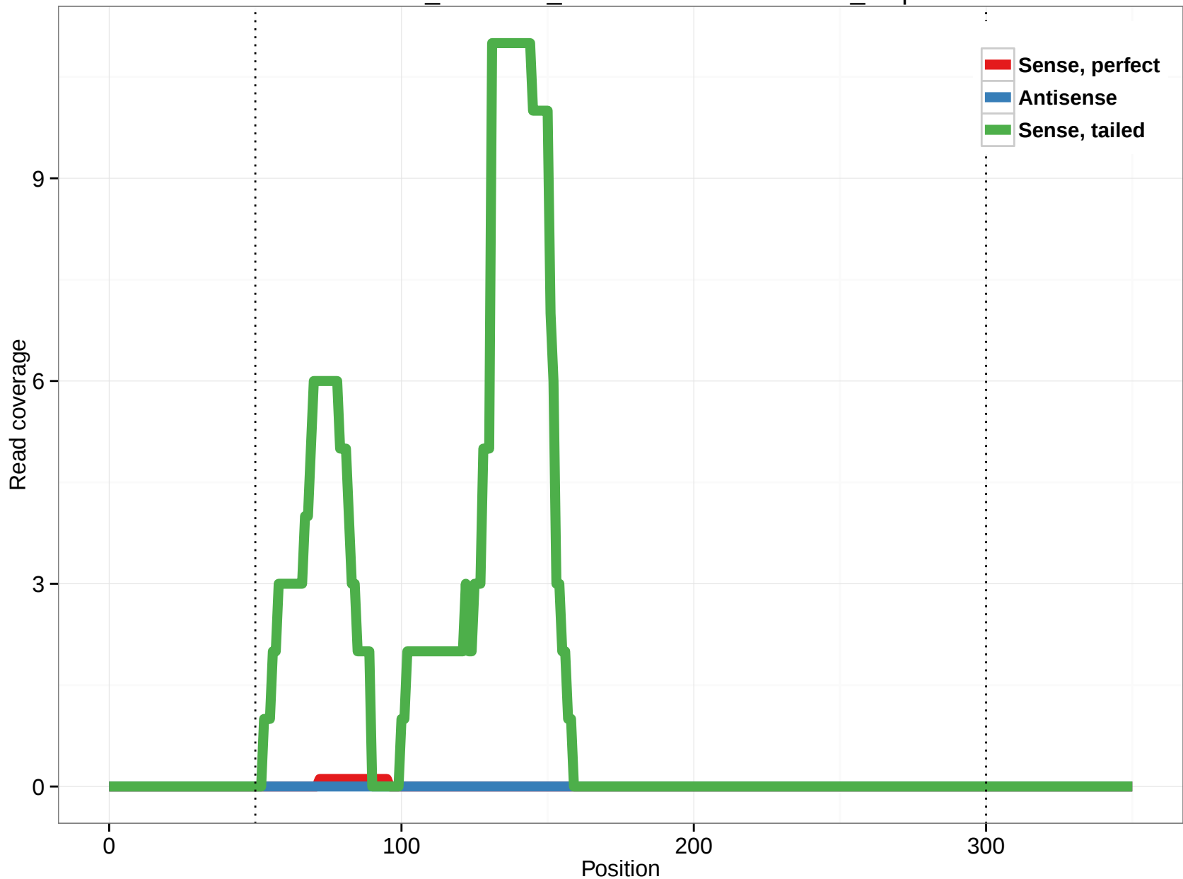
ornAna1_ensGene_ENSOANT00000012273_2.5p
