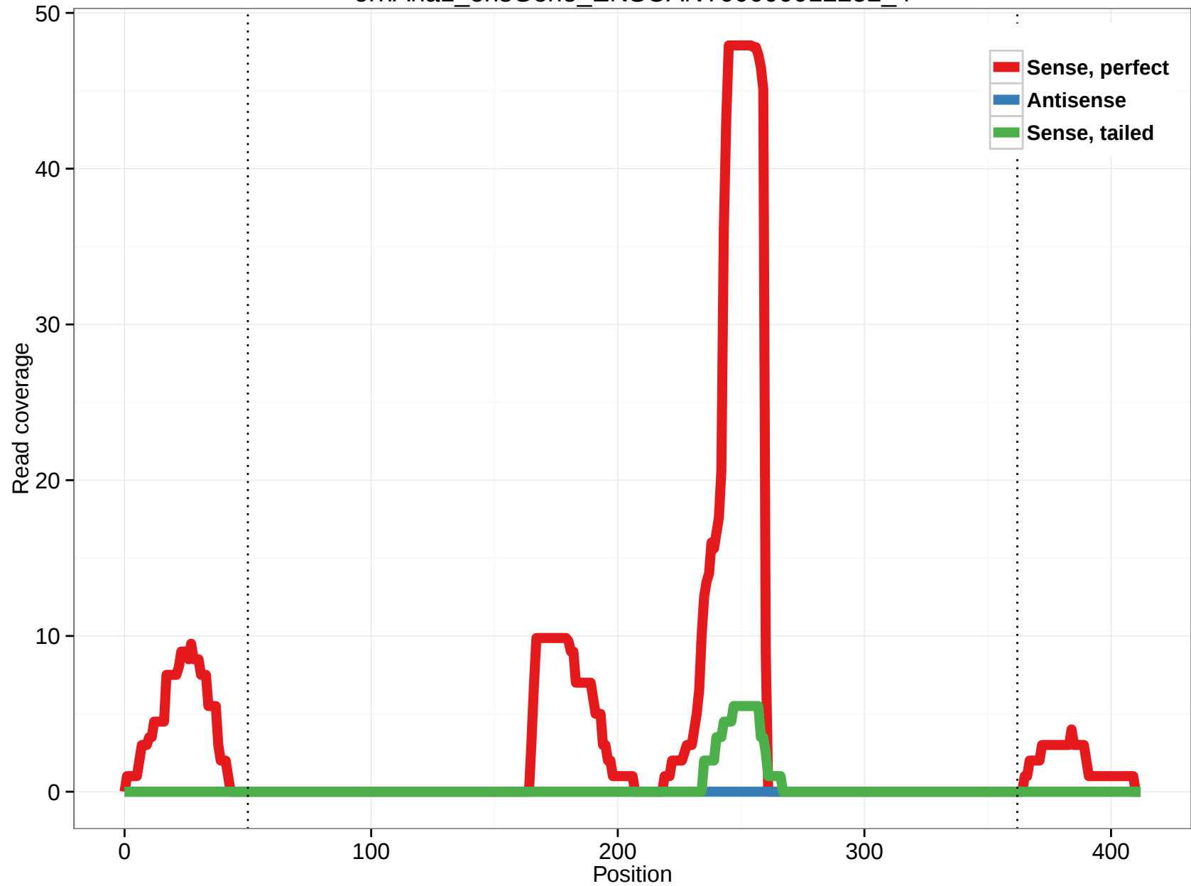
ornAna1_ensGene_ENSOANT00000012252_4
