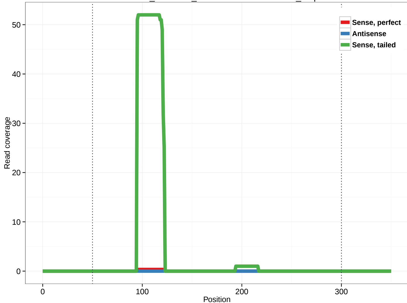
ornAna1_ensGene_ENSOANT00000012239_7.5p
