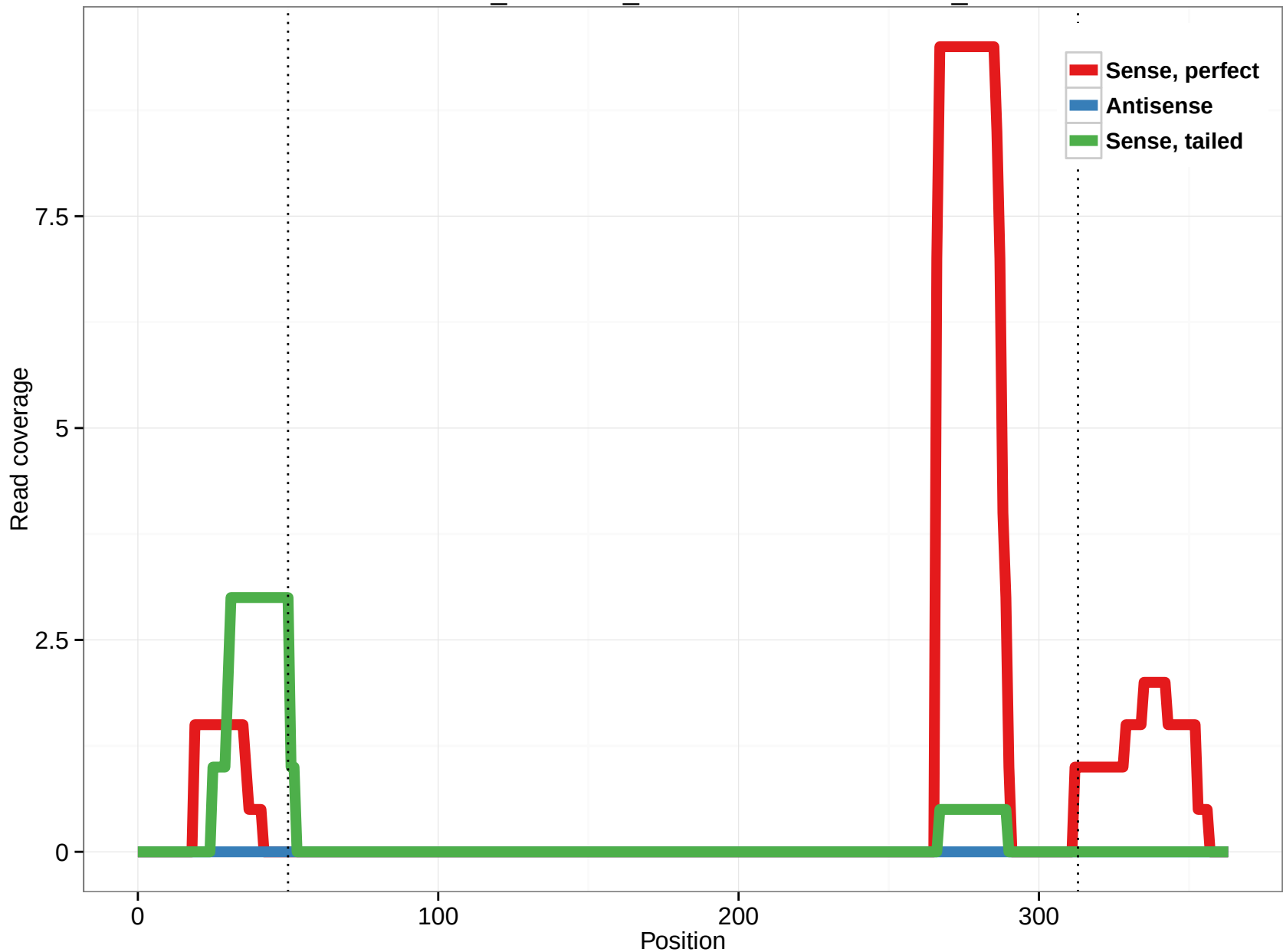
ornAna1_ensGene_ENSOANT00000012226_0
