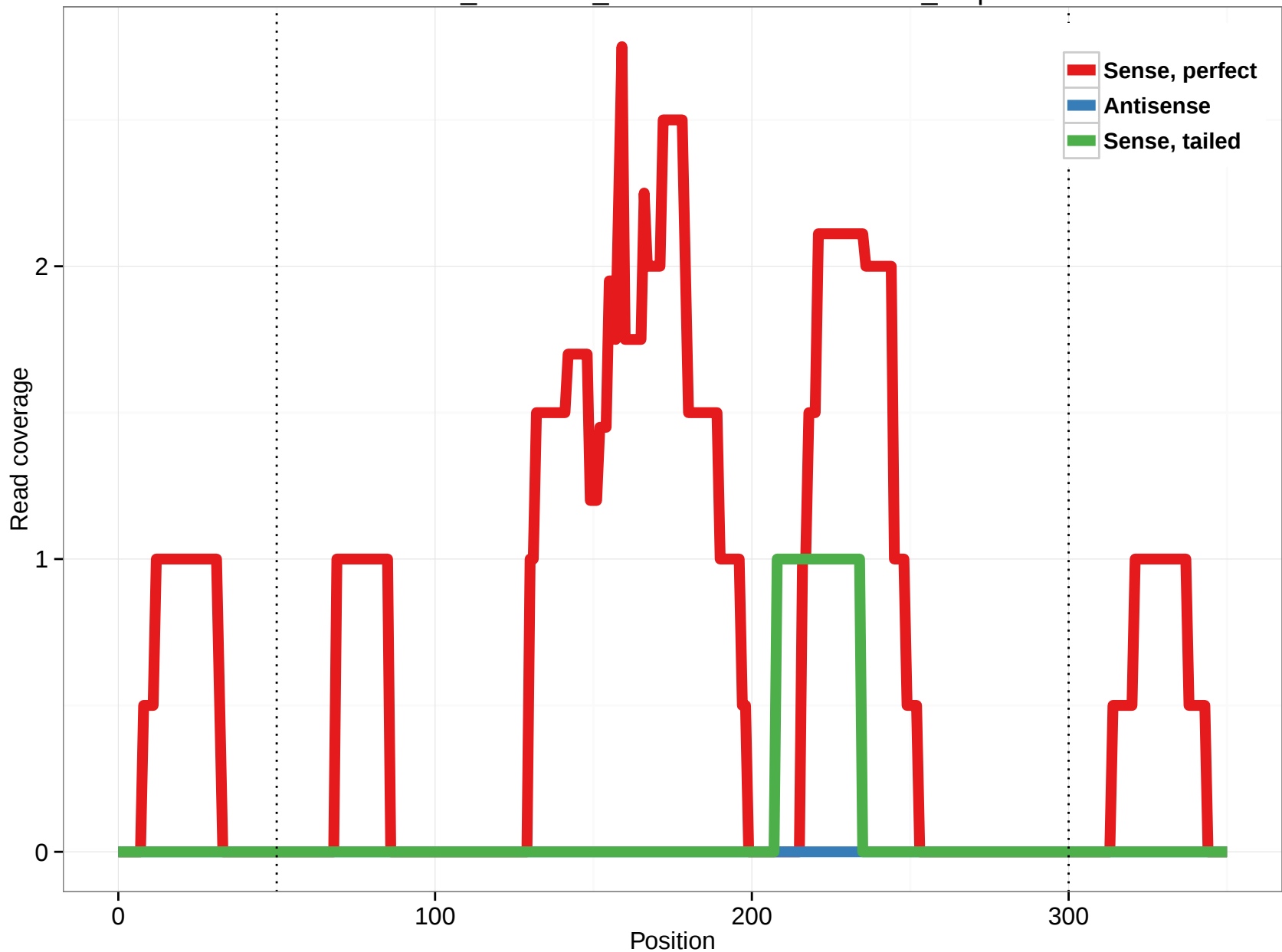
ornAna1_ensGene_ENSOANT00000012217_4.5p
