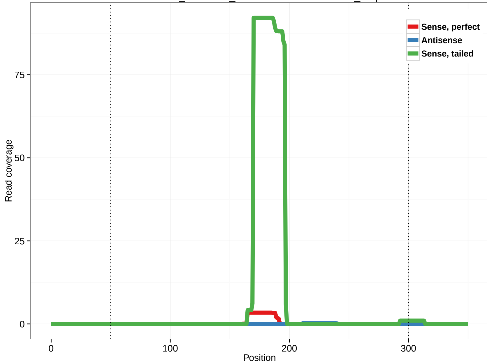
ornAna1_ensGene_ENSOANT00000012180_0.5p
