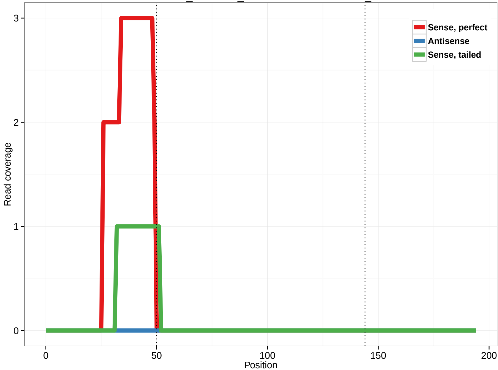
ornAna1_ensGene_ENSOANT00000012165_2
