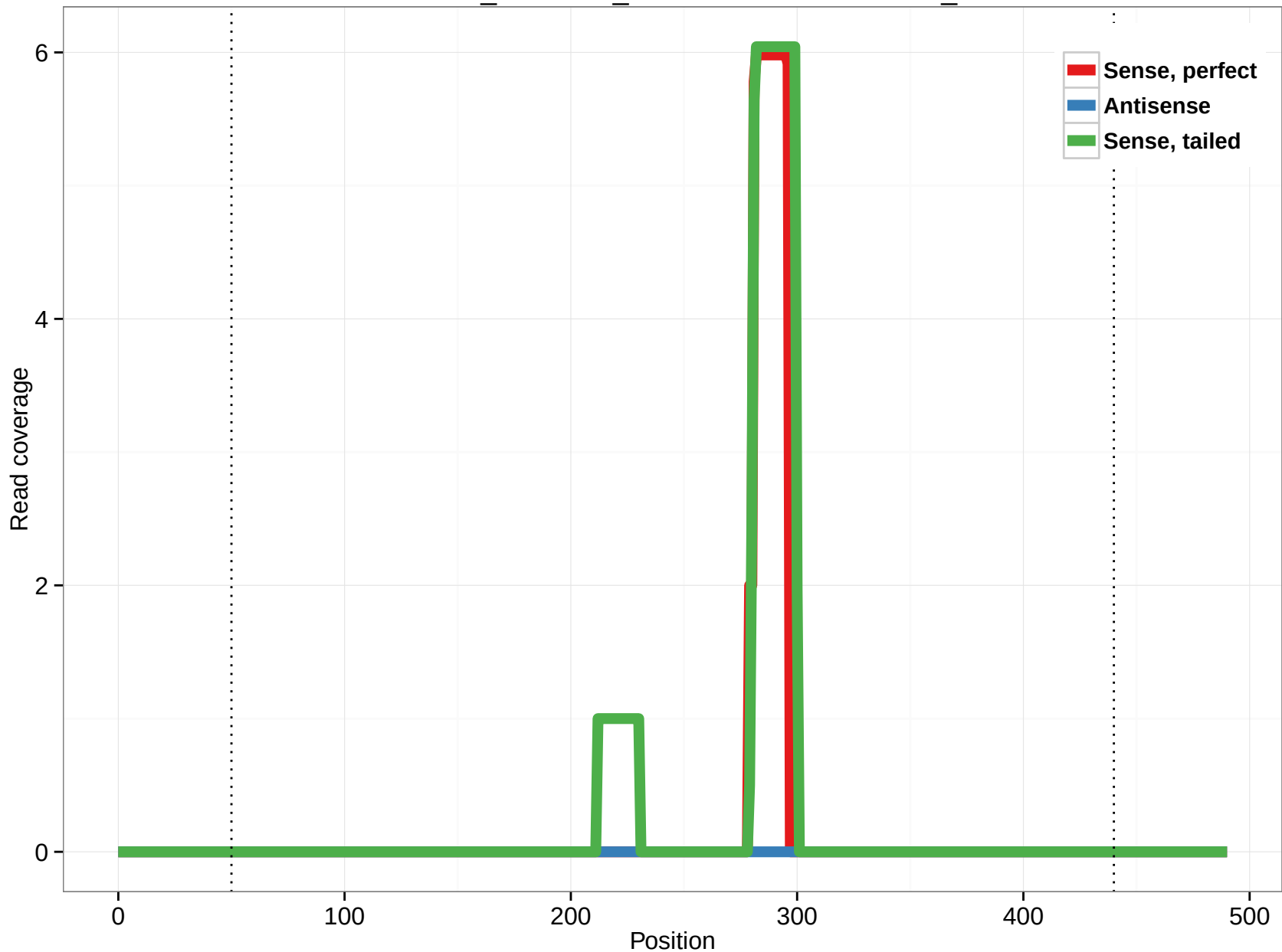
ornAna1_ensGene_ENSOANT00000012120_1
