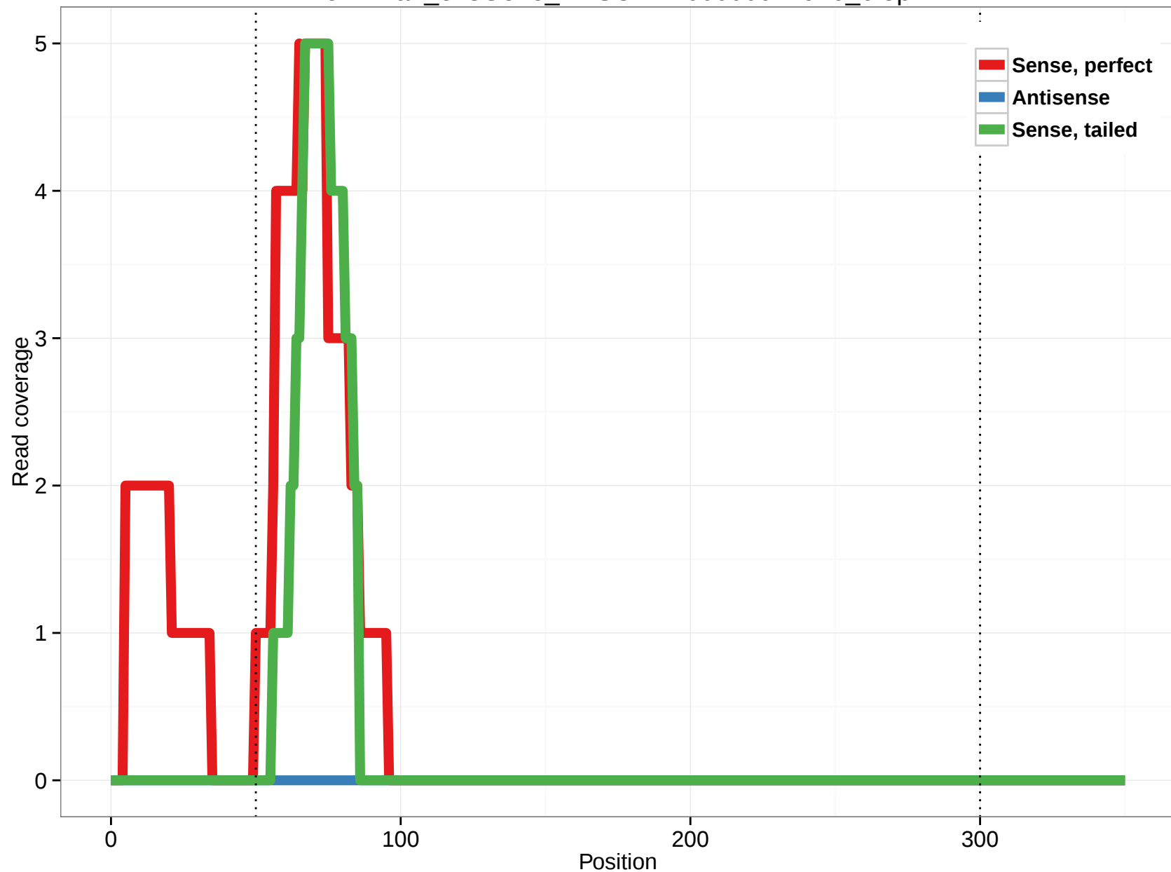
ornAna1_ensGene_ENSOANT00000011916_6.5p
