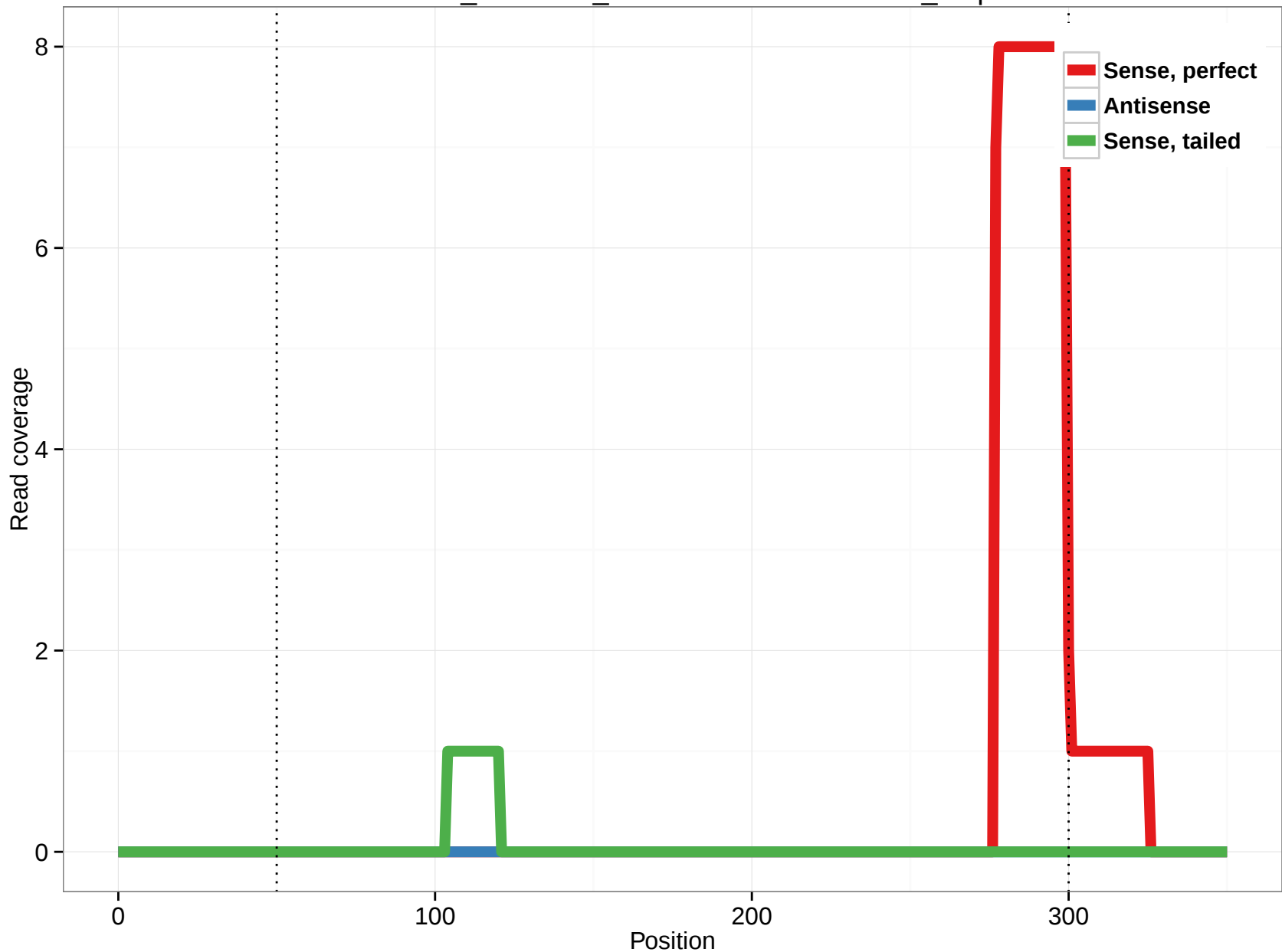
ornAna1_ensGene_ENSOANT00000011851_5.3p
