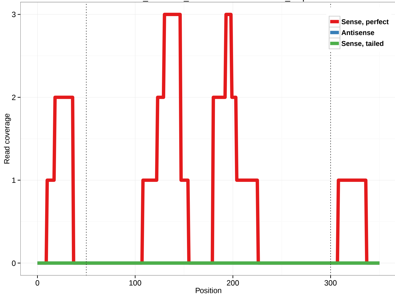
ornAna1_ensGene_ENSOANT00000011818_8.5p
